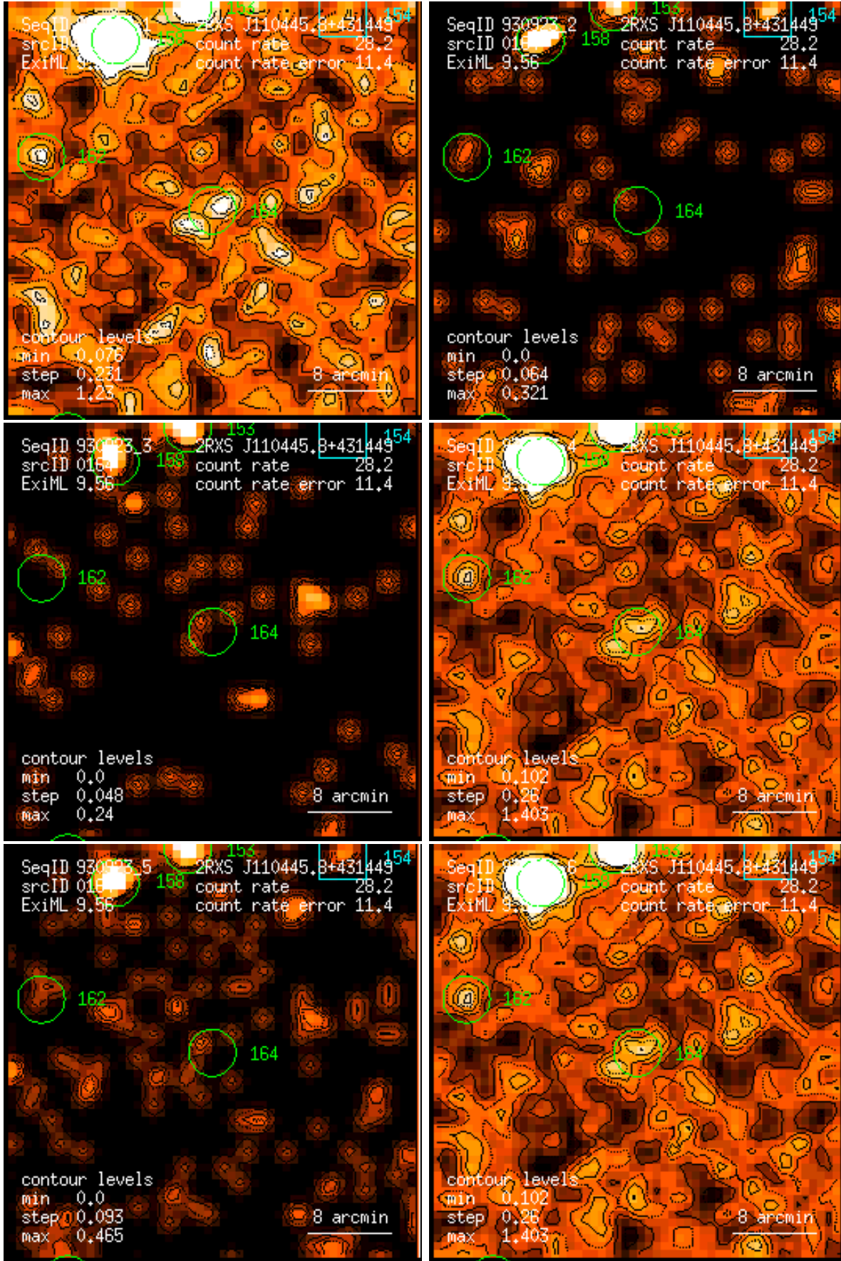
Figure 164: RASS 930923: detection 0164: band rate images, Gaussian filter: (1) PSPC channels 11 – 41, (2) 52 – 90, (3) 91 – 201, (4) 11 – 235, (5) 52 – 201, (6) 11 – 201. Broad band rates in counts/ks. Band rate contour levels in counts/ks/arcmin 2 .
