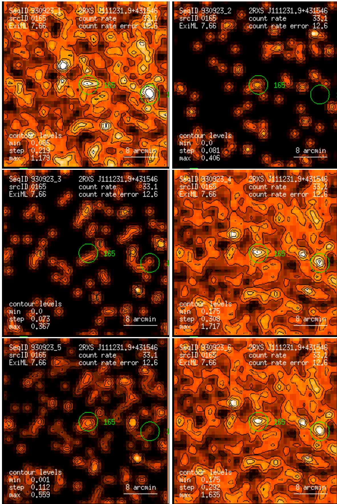
Figure 165: RASS 930923: detection 0165: band rate images, Gaussian filter: (1) PSPC channels 11 – 41, (2) 52 – 90, (3) 91 – 201, (4) 11 – 235, (5) 52 – 201, (6) 11 – 201. Broad band rates in counts/ks. Band rate contour levels in counts/ks/arcmin 2 .
