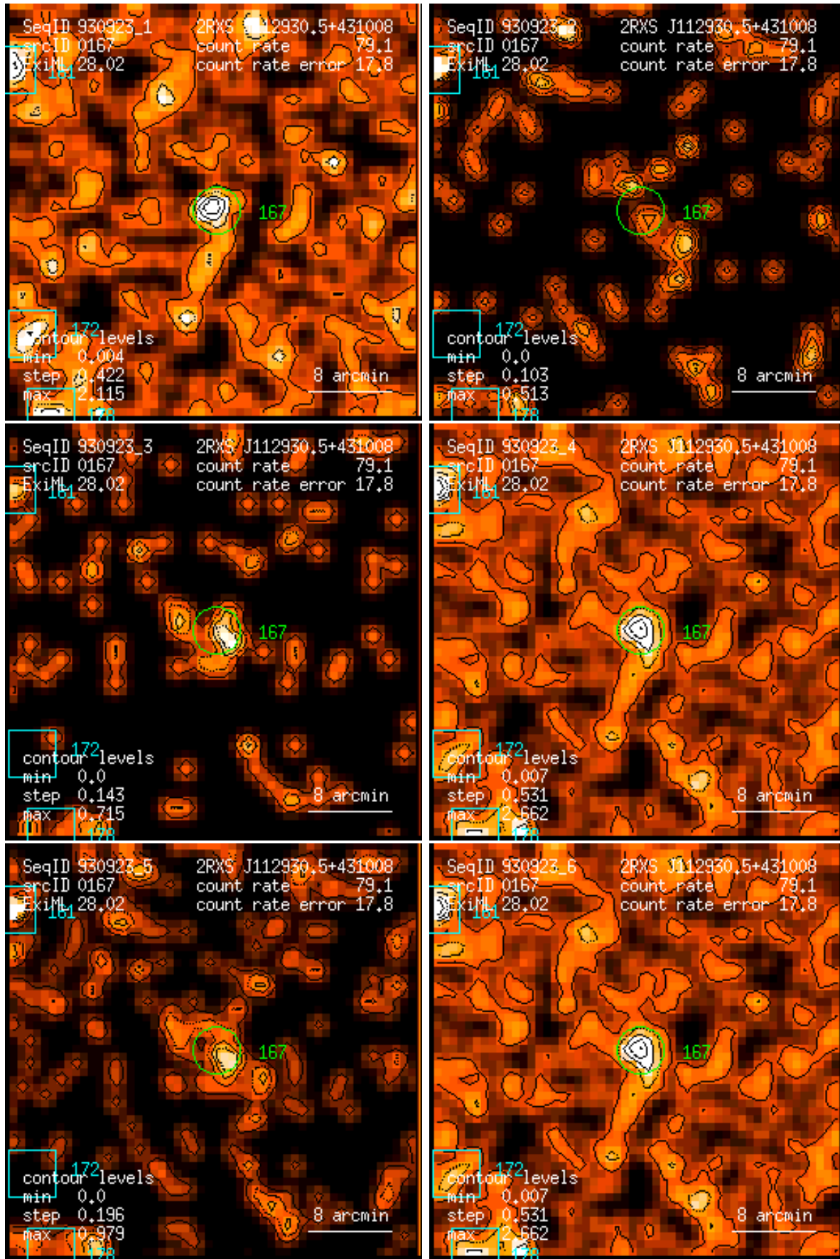
Figure 167: RASS 930923: detection 0167: band rate images, Gaussian filter: (1) PSPC channels 11 – 41, (2) 52 – 90, (3) 91 – 201, (4) 11 – 235, (5) 52 – 201, (6) 11 – 201. Broad band rates in counts/ks. Band rate contour levels in counts/ks/arcmin 2 .
