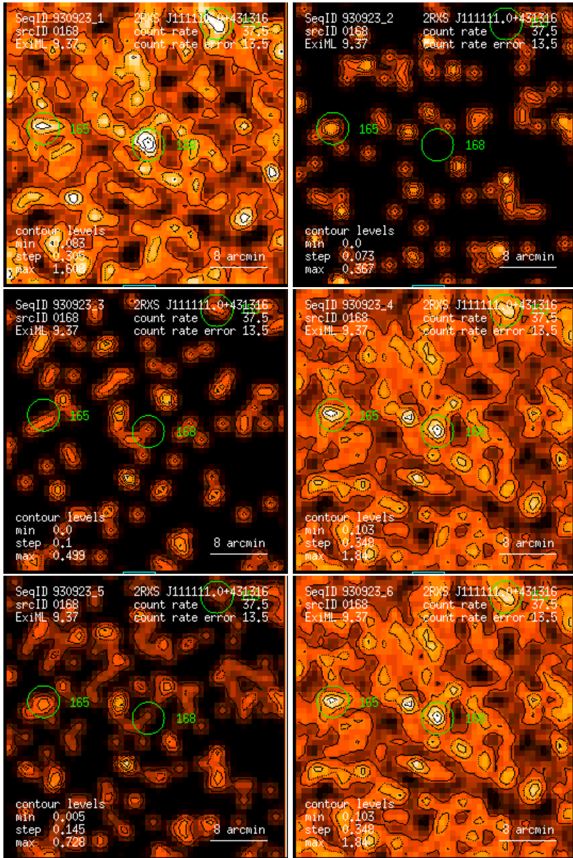
Figure 168: RASS 930923: detection 0168: band rate images, Gaussian filter: (1) PSPC channels 11 – 41, (2) 52 – 90, (3) 91 – 201, (4) 11 – 235, (5) 52 – 201, (6) 11 – 201. Broad band rates in counts/ks. Band rate contour levels in counts/ks/arcmin 2 .
