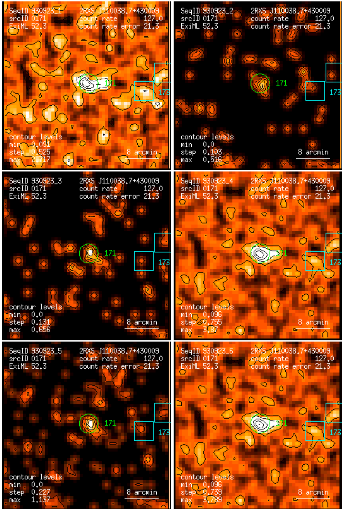
Figure 171: RASS 930923: detection 0171: band rate images, Gaussian filter: (1) PSPC channels 11 – 41, (2) 52 – 90, (3) 91 – 201, (4) 11 – 235, (5) 52 – 201, (6) 11 – 201. Broad band rates in counts/ks. Band rate contour levels in counts/ks/arcmin 2 .
