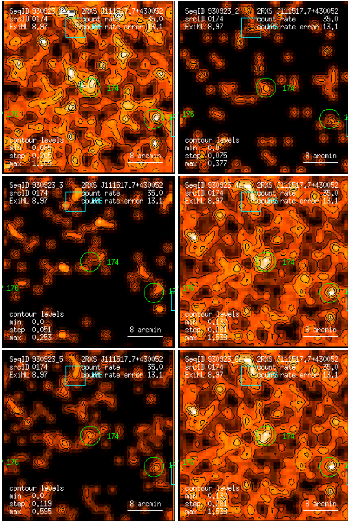
Figure 174: RASS 930923: detection 0174: band rate images, Gaussian filter: (1) PSPC channels 11 – 41, (2) 52 – 90, (3) 91 – 201, (4) 11 – 235, (5) 52 – 201, (6) 11 – 201. Broad band rates in counts/ks. Band rate contour levels in counts/ks/arcmin 2 .
