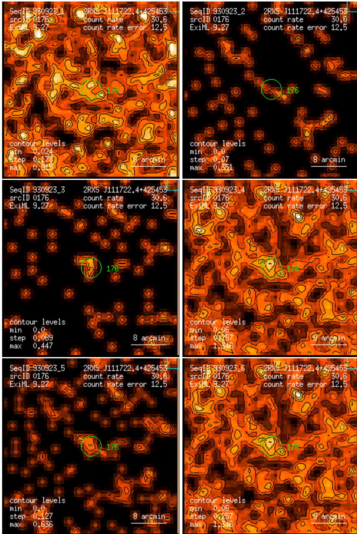
Figure 176: RASS 930923: detection 0176: band rate images, Gaussian filter: (1) PSPC channels 11 – 41, (2) 52 – 90, (3) 91 – 201, (4) 11 – 235, (5) 52 – 201, (6) 11 – 201. Broad band rates in counts/ks. Band rate contour levels in counts/ks/arcmin 2 .
