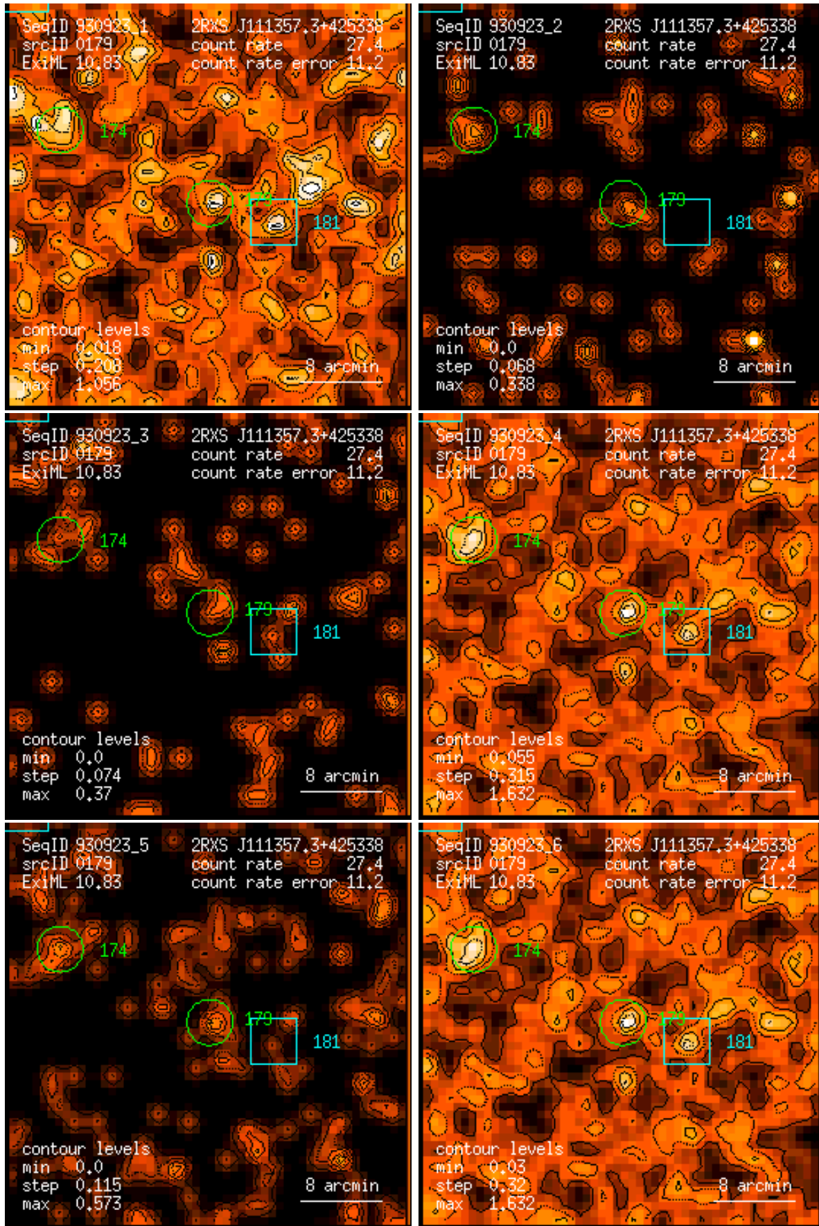
Figure 179: RASS 930923: detection 0179: band rate images, Gaussian filter: (1) PSPC channels 11 – 41, (2) 52 – 90, (3) 91 – 201, (4) 11 – 235, (5) 52 – 201, (6) 11 – 201. Broad band rates in counts/ks. Band rate contour levels in counts/ks/arcmin 2 .
