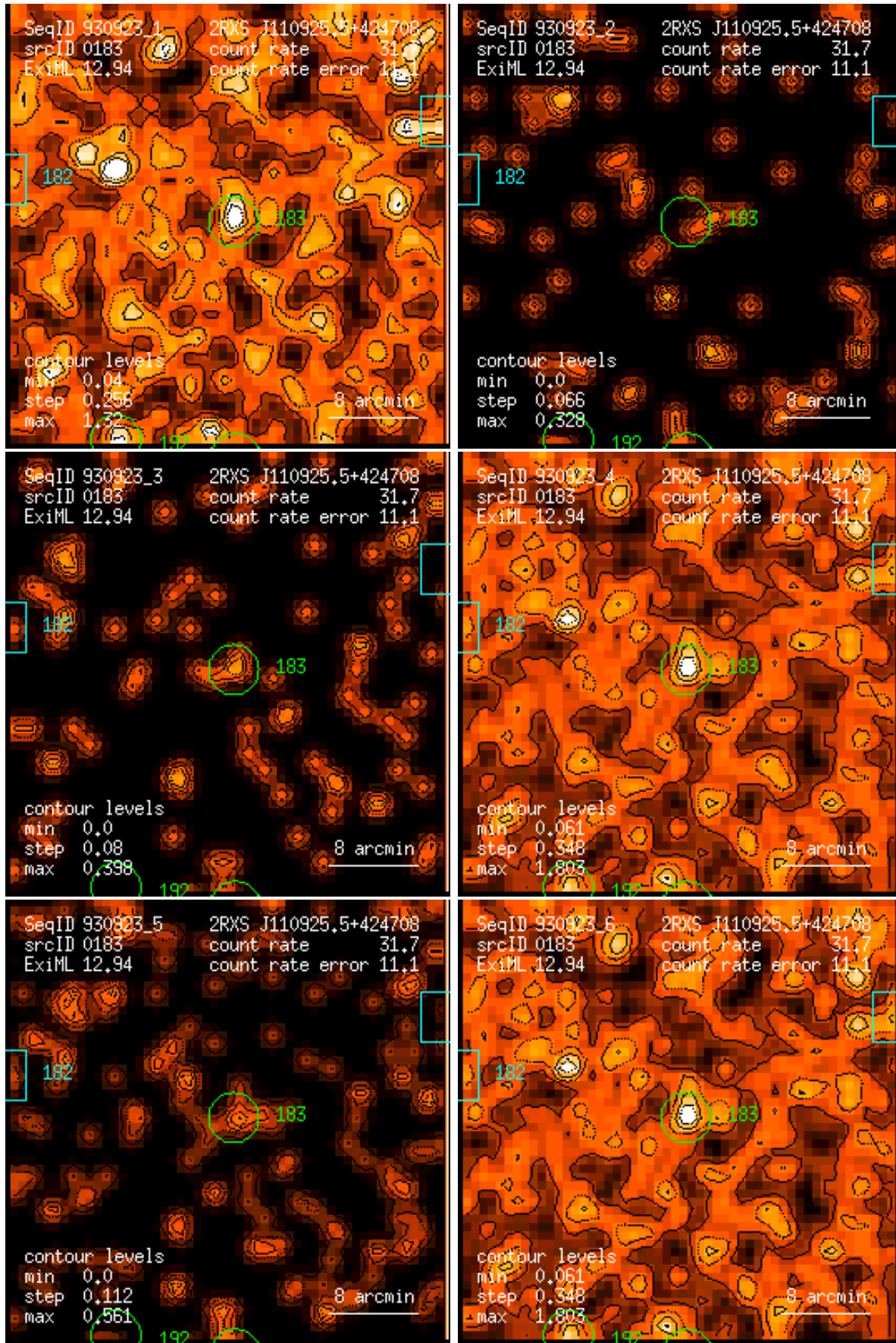
Figure 183: RASS 930923: detection 0183: band rate images, Gaussian filter: (1) PSPC channels 11 – 41, (2) 52 – 90, (3) 91 – 201, (4) 11 – 235, (5) 52 – 201, (6) 11 – 201. Broad band rates in counts/ks. Band rate contour levels in counts/ks/arcmin 2 .
