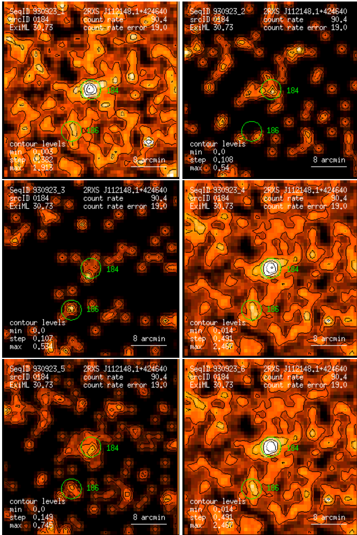
Figure 184: RASS 930923: detection 0184: band rate images, Gaussian filter: (1) PSPC channels 11 – 41, (2) 52 – 90, (3) 91 – 201, (4) 11 – 235, (5) 52 – 201, (6) 11 – 201. Broad band rates in counts/ks. Band rate contour levels in counts/ks/arcmin 2 .
