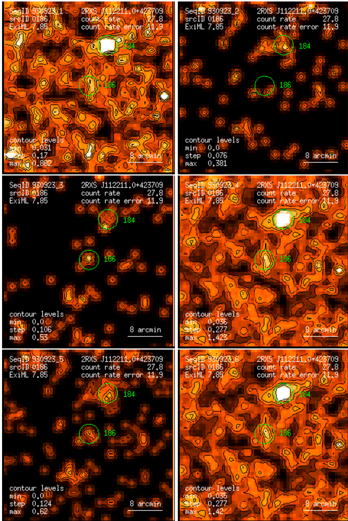
Figure 186: RASS 930923: detection 0186: band rate images, Gaussian filter: (1) PSPC channels 11 – 41, (2) 52 – 90, (3) 91 – 201, (4) 11 – 235, (5) 52 – 201, (6) 11 – 201. Broad band rates in counts/ks. Band rate contour levels in counts/ks/arcmin 2 .
