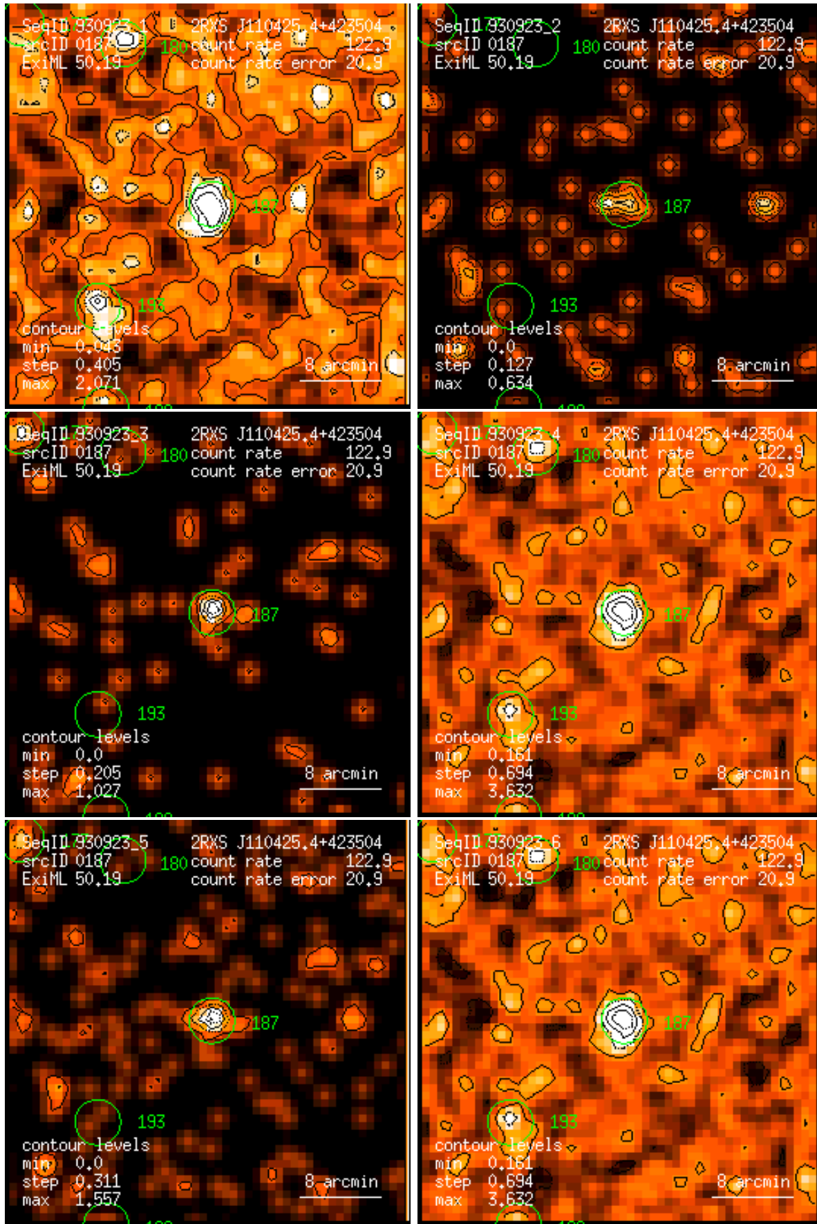
Figure 187: RASS 930923: detection 0187: band rate images, Gaussian filter: (1) PSPC channels 11 – 41, (2) 52 – 90, (3) 91 – 201, (4) 11 – 235, (5) 52 – 201, (6) 11 – 201. Broad band rates in counts/ks. Band rate contour levels in counts/ks/arcmin 2 .
