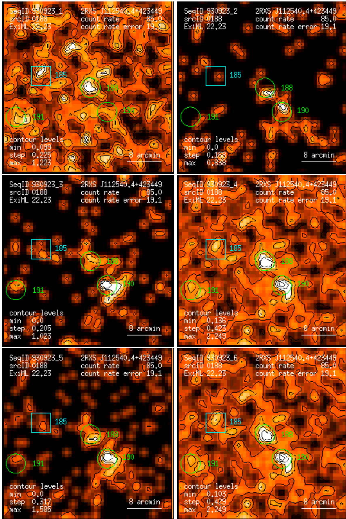
Figure 188: RASS 930923: detection 0188: band rate images, Gaussian filter: (1) PSPC channels 11 – 41, (2) 52 – 90, (3) 91 – 201, (4) 11 – 235, (5) 52 – 201, (6) 11 – 201. Broad band rates in counts/ks. Band rate contour levels in counts/ks/arcmin 2 .
