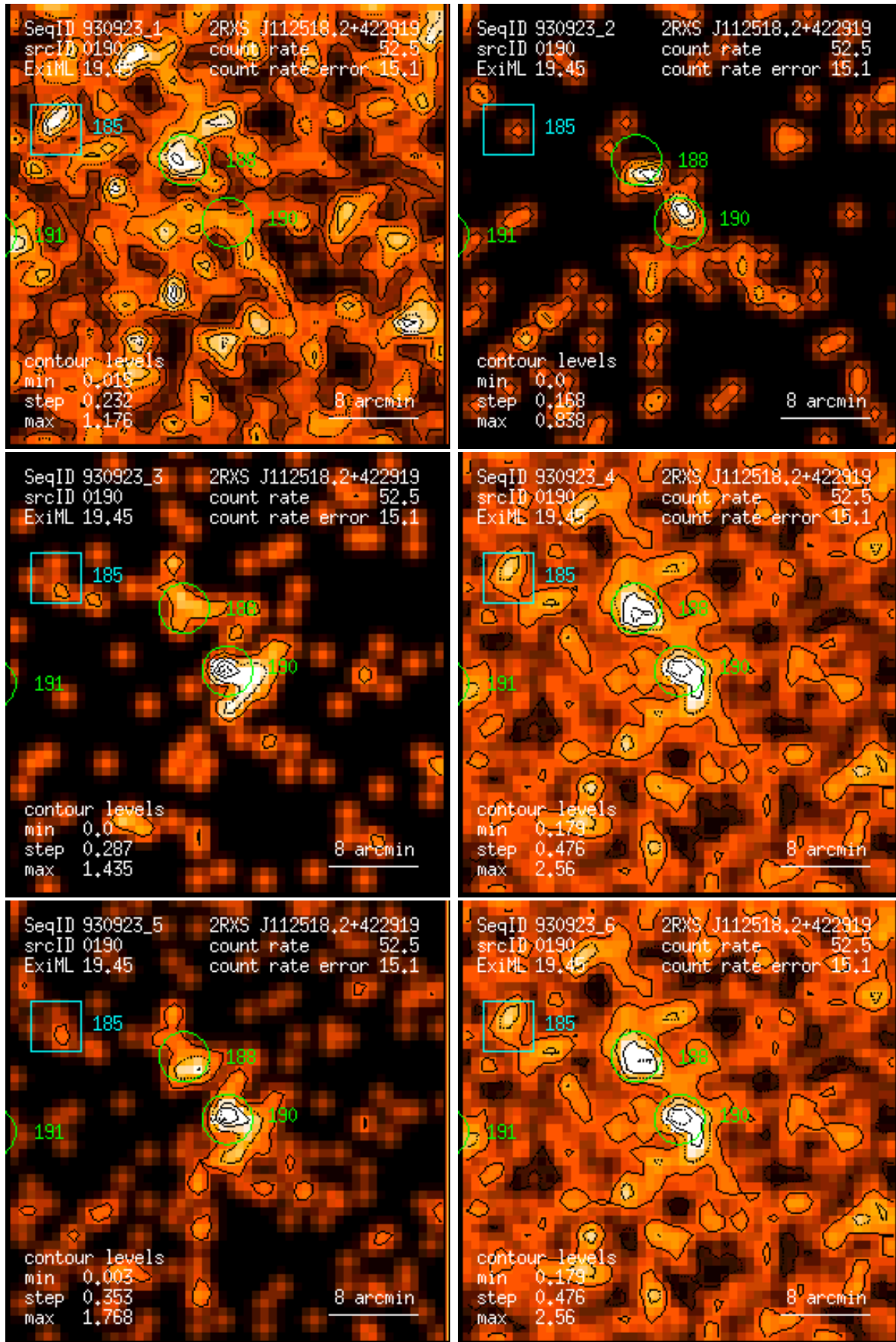
Figure 190: RASS 930923: detection 0190: band rate images, Gaussian filter: (1) PSPC channels 11 – 41, (2) 52 – 90, (3) 91 – 201, (4) 11 – 235, (5) 52 – 201, (6) 11 – 201. Broad band rates in counts/ks. Band rate contour levels in counts/ks/arcmin 2 .
