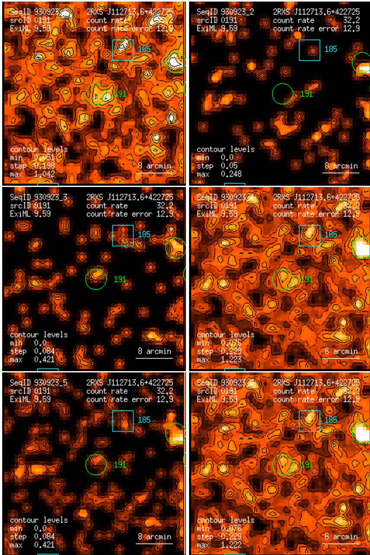
Figure 191: RASS 930923: detection 0191: band rate images, Gaussian filter: (1) PSPC channels 11 – 41, (2) 52 – 90, (3) 91 – 201, (4) 11 – 235, (5) 52 – 201, (6) 11 – 201. Broad band rates in counts/ks. Band rate contour levels in counts/ks/arcmin 2 .
