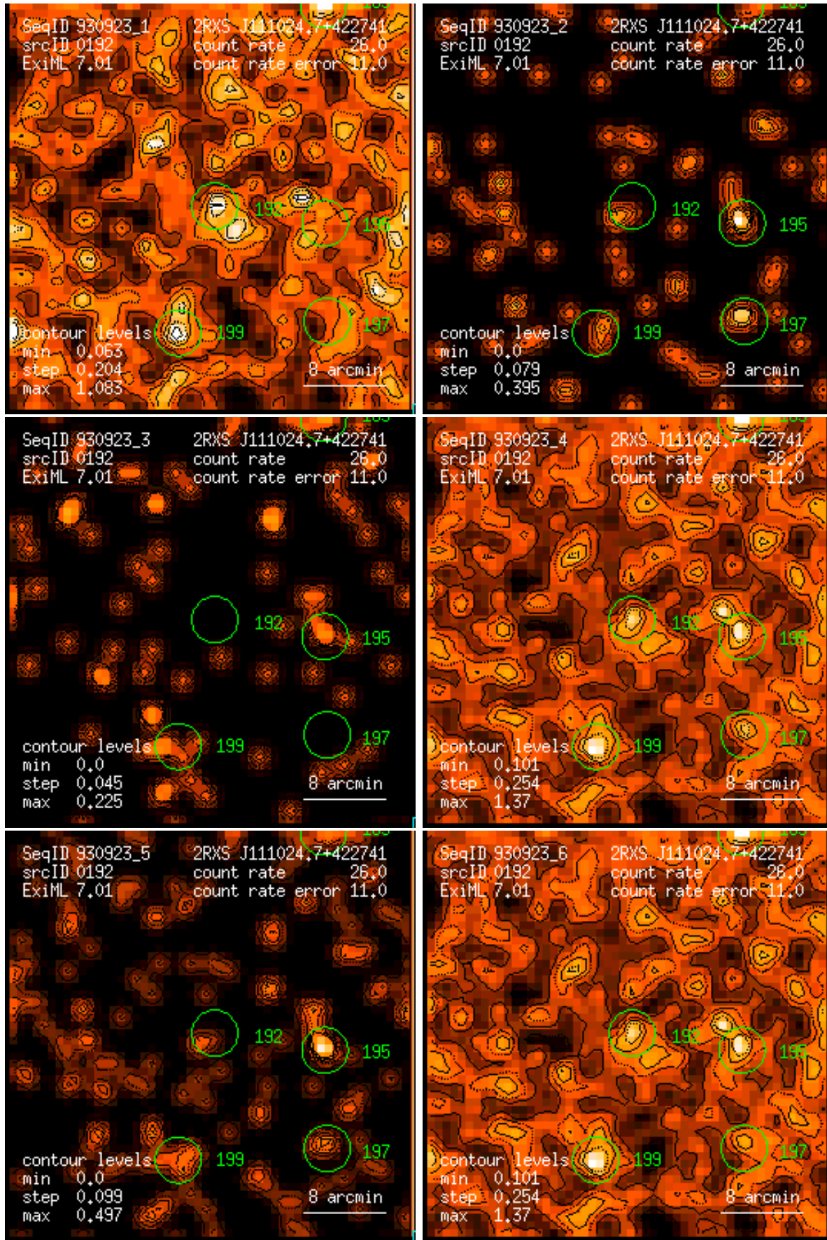
Figure 192: RASS 930923: detection 0192: band rate images, Gaussian filter: (1) PSPC channels 11 – 41, (2) 52 – 90, (3) 91 – 201, (4) 11 – 235, (5) 52 – 201, (6) 11 – 201. Broad band rates in counts/ks. Band rate contour levels in counts/ks/arcmin 2 .
