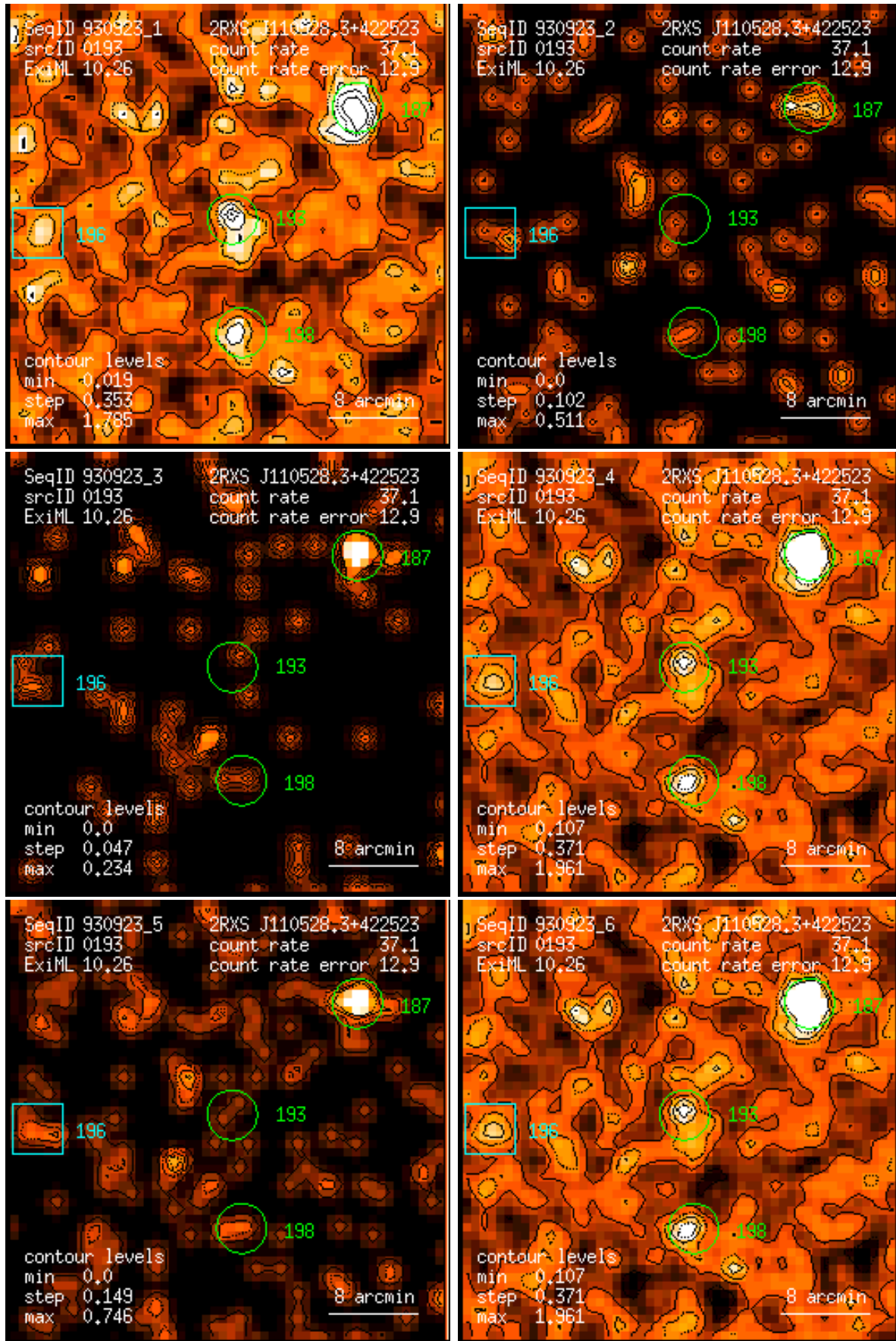
Figure 193: RASS 930923: detection 0193: band rate images, Gaussian filter: (1) PSPC channels 11 – 41, (2) 52 – 90, (3) 91 – 201, (4) 11 – 235, (5) 52 – 201, (6) 11 – 201. Broad band rates in counts/ks. Band rate contour levels in counts/ks/arcmin 2 .
