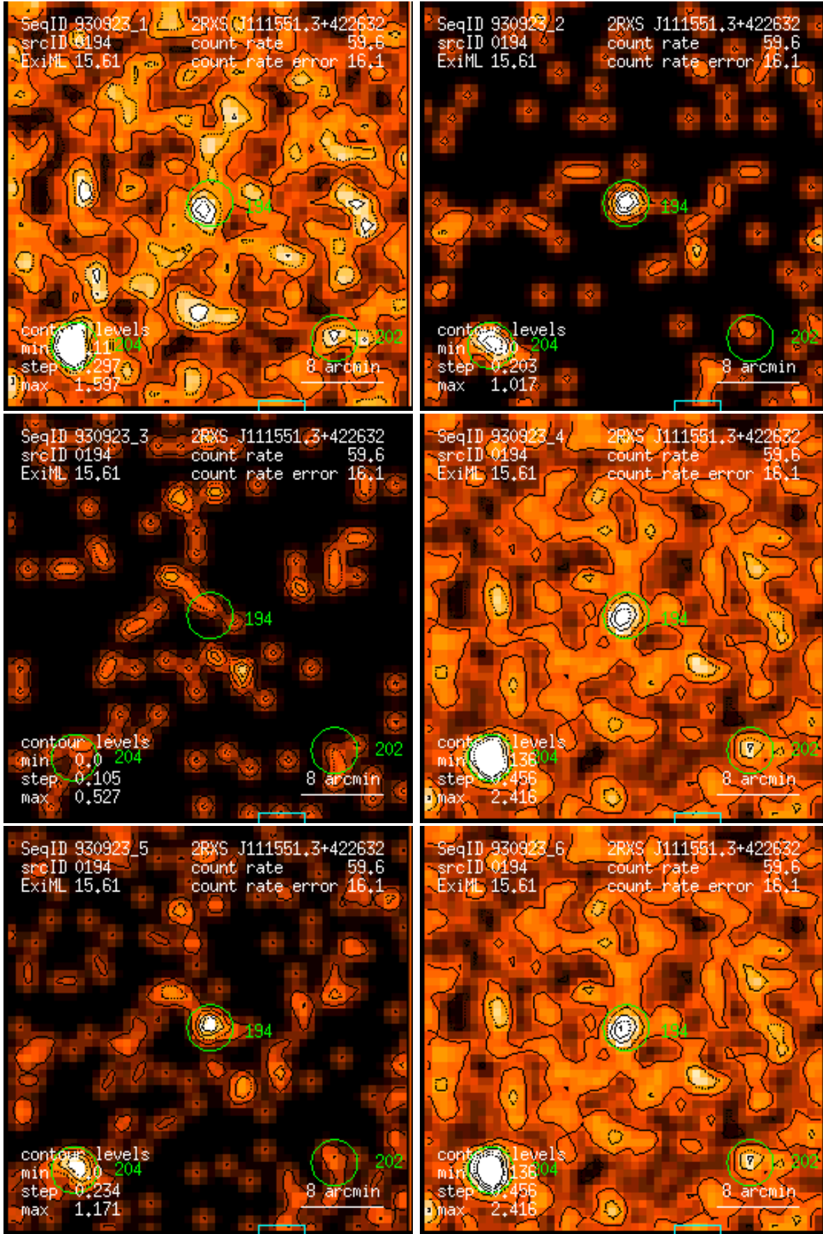
Figure 194: RASS 930923: detection 0194: band rate images, Gaussian filter: (1) PSPC channels 11 – 41, (2) 52 – 90, (3) 91 – 201, (4) 11 – 235, (5) 52 – 201, (6) 11 – 201. Broad band rates in counts/ks. Band rate contour levels in counts/ks/arcmin 2 .
