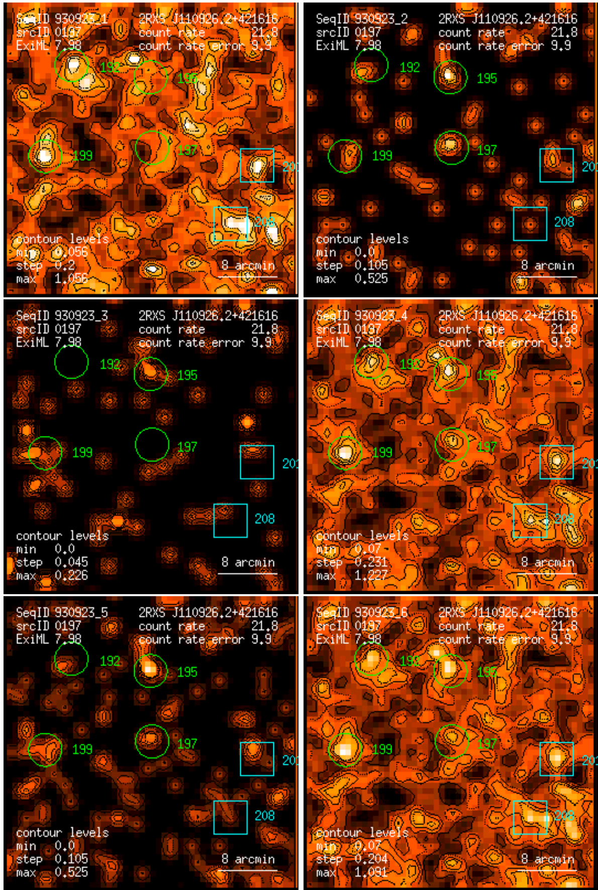
Figure 197: RASS 930923: detection 0197: band rate images, Gaussian filter: (1) PSPC channels 11 – 41, (2) 52 – 90, (3) 91 – 201, (4) 11 – 235, (5) 52 – 201, (6) 11 – 201. Broad band rates in counts/ks. Band rate contour levels in counts/ks/arcmin 2 .
