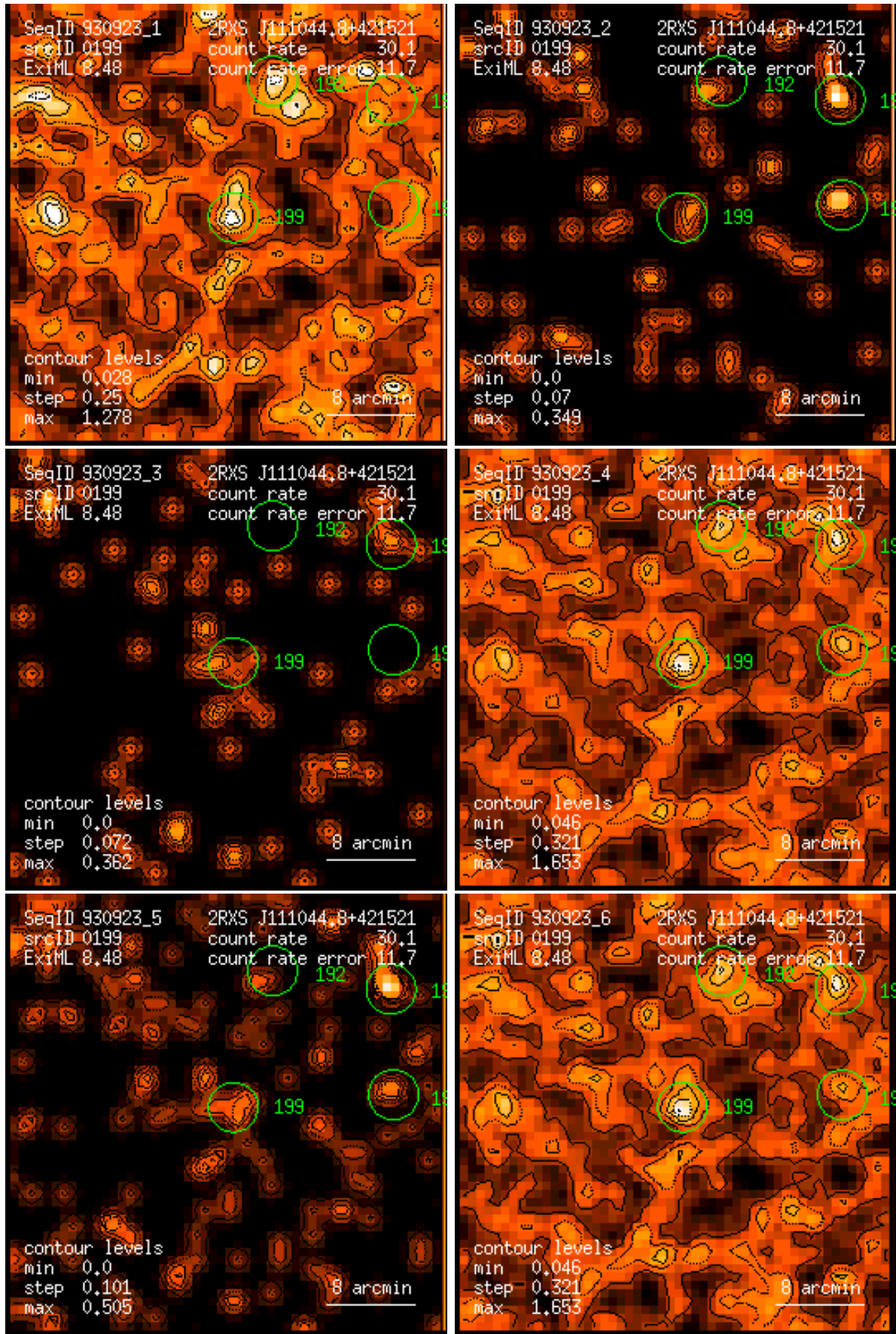
Figure 199: RASS 930923: detection 0199: band rate images, Gaussian filter: (1) PSPC channels 11 – 41, (2) 52 – 90, (3) 91 – 201, (4) 11 – 235, (5) 52 – 201, (6) 11 – 201. Broad band rates in counts/ks. Band rate contour levels in counts/ks/arcmin 2 .
