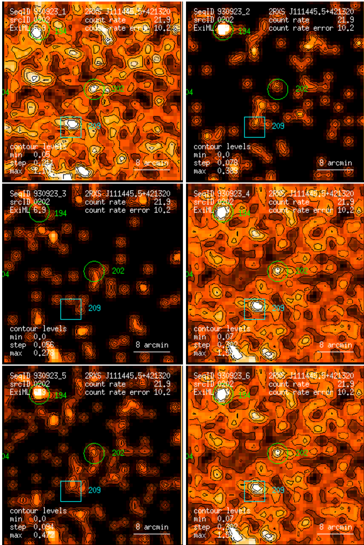
Figure 202: RASS 930923: detection 0202: band rate images, Gaussian filter: (1) PSPC channels 11 – 41, (2) 52 – 90, (3) 91 – 201, (4) 11 – 235, (5) 52 – 201, (6) 11 – 201. Broad band rates in counts/ks. Band rate contour levels in counts/ks/arcmin 2 .
