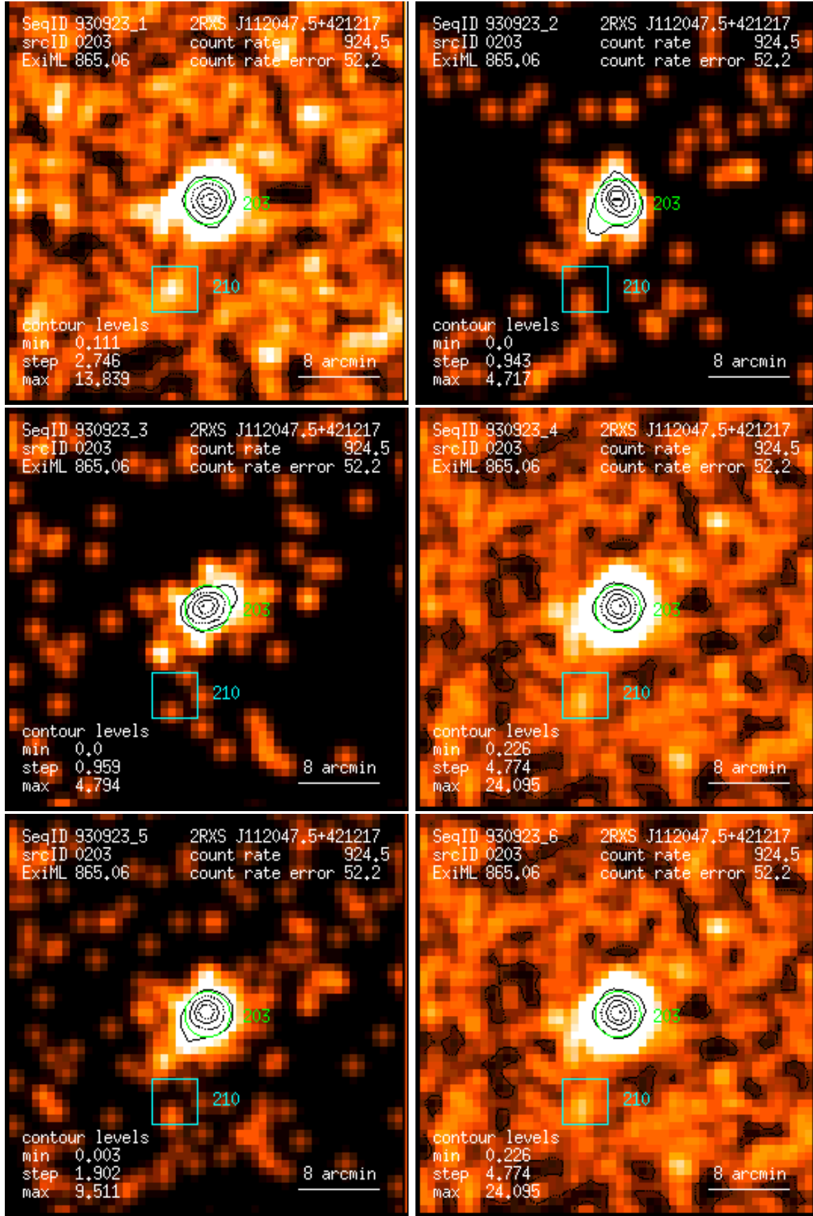
Figure 203: RASS 930923: detection 0203: band rate images, Gaussian filter: (1) PSPC channels 11 – 41, (2) 52 – 90, (3) 91 – 201, (4) 11 – 235, (5) 52 – 201, (6) 11 – 201. Broad band rates in counts/ks. Band rate contour levels in counts/ks/arcmin 2 .
