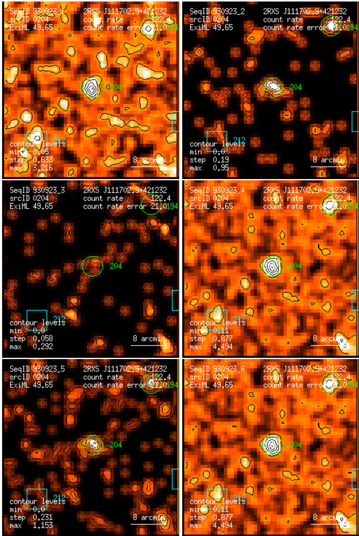
Figure 204: RASS 930923: detection 0204: band rate images, Gaussian filter: (1) PSPC channels 11 – 41, (2) 52 – 90, (3) 91 – 201, (4) 11 – 235, (5) 52 – 201, (6) 11 – 201. Broad band rates in counts/ks. Band rate contour levels in counts/ks/arcmin 2 .
