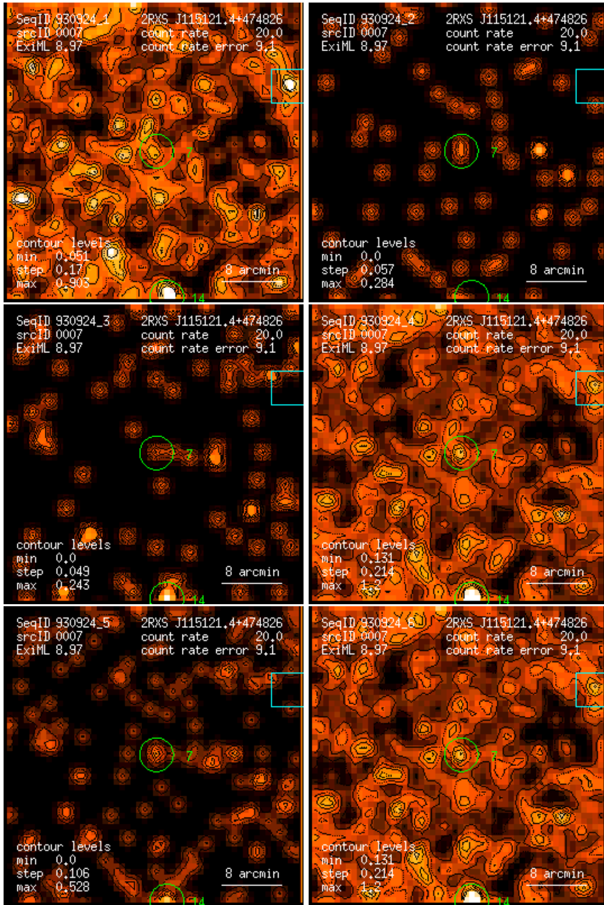
Figure 7: RASS 930924: detection 0007: band rate images, Gaussian filter: (1) PSPC channels 11 – 41, (2) 52 – 90, (3) 91 – 201, (4) 11 – 235, (5) 52 – 201, (6) 11 – 201. Broad band rates in counts/ks. Band rate contour levels in counts/ks/arcmin 2 .
