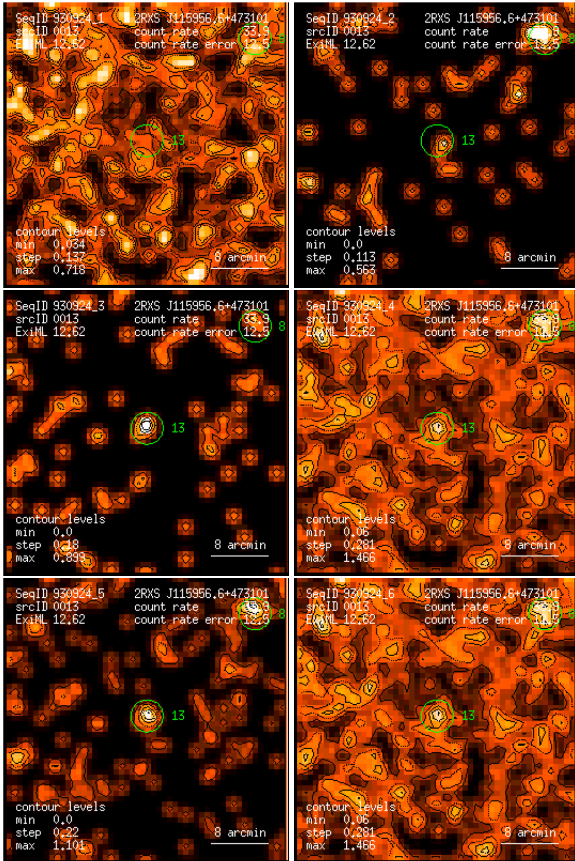
Figure 13: RASS 930924: detection 0013: band rate images, Gaussian filter: (1) PSPC channels 11 – 41, (2) 52 – 90, (3) 91 – 201, (4) 11 – 235, (5) 52 – 201, (6) 11 – 201. Broad band rates in counts/ks. Band rate contour levels in counts/ks/arcmin 2 .
