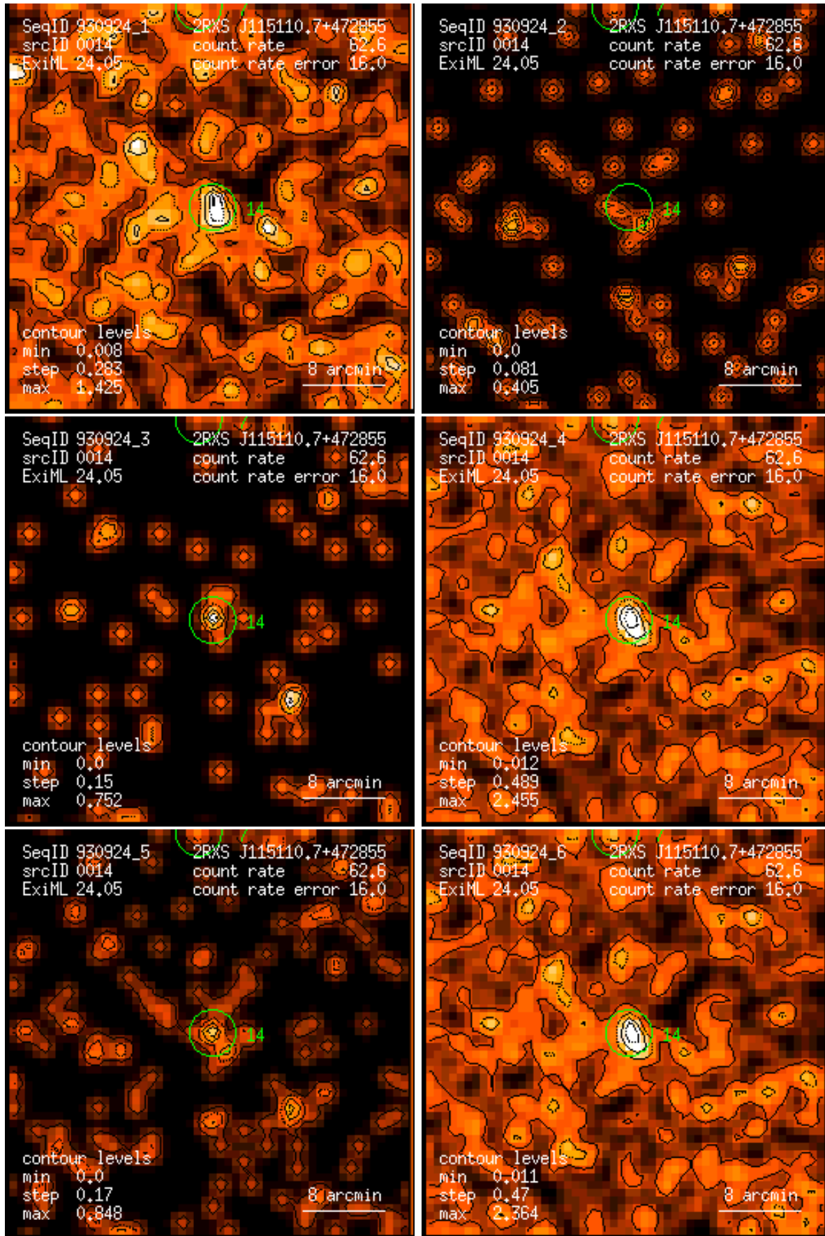
Figure 14: RASS 930924: detection 0014: band rate images, Gaussian filter: (1) PSPC channels 11 – 41, (2) 52 – 90, (3) 91 – 201, (4) 11 – 235, (5) 52 – 201, (6) 11 – 201. Broad band rates in counts/ks. Band rate contour levels in counts/ks/arcmin 2 .
