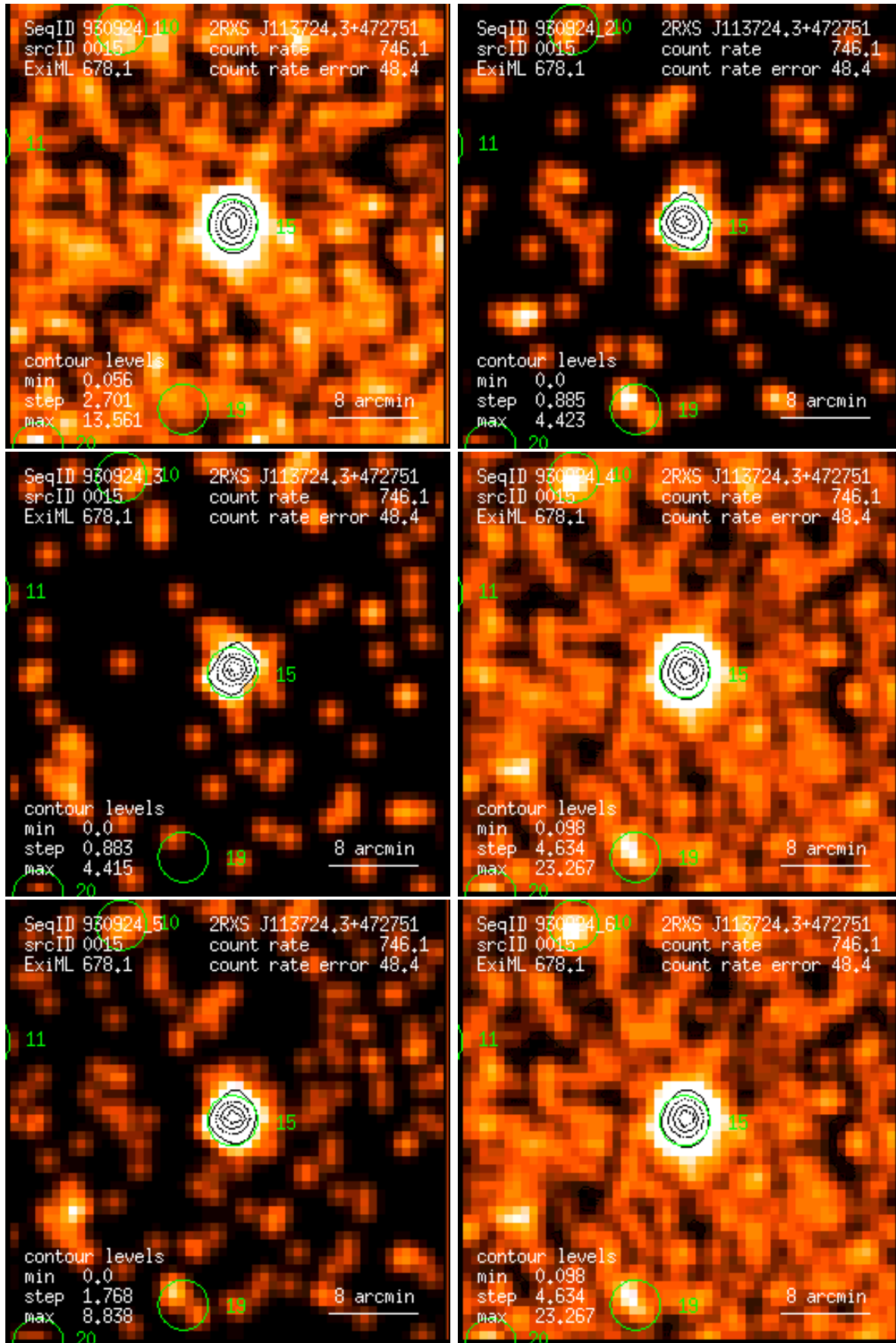
Figure 15: RASS 930924: detection 0015: band rate images, Gaussian filter: (1) PSPC channels 11 – 41, (2) 52 – 90, (3) 91 – 201, (4) 11 – 235, (5) 52 – 201, (6) 11 – 201. Broad band rates in counts/ks. Band rate contour levels in counts/ks/arcmin 2 .
