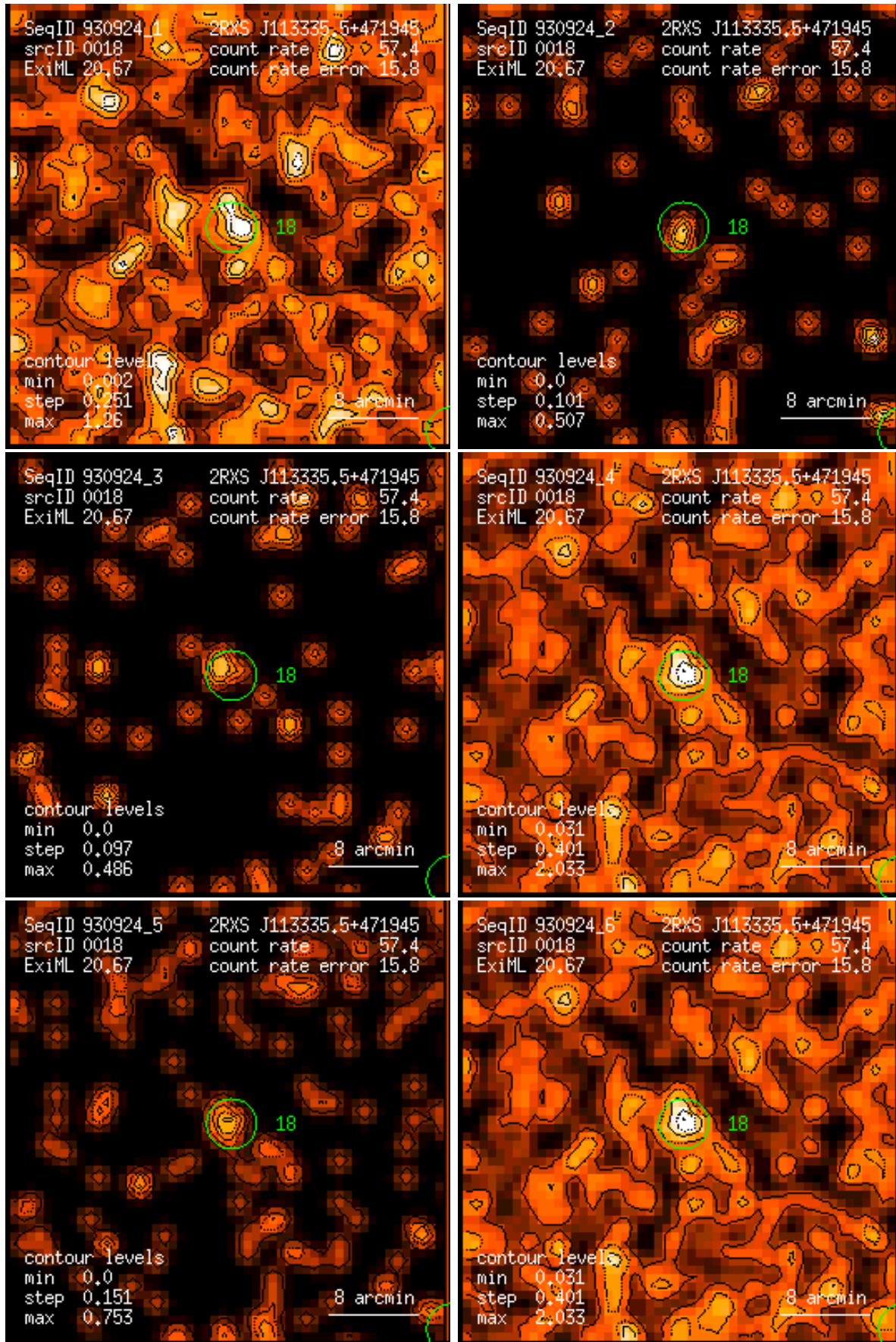
Figure 18: RASS 930924: detection 0018: band rate images, Gaussian filter: (1) PSPC channels 11 – 41, (2) 52 – 90, (3) 91 – 201, (4) 11 – 235, (5) 52 – 201, (6) 11 – 201. Broad band rates in counts/ks. Band rate contour levels in counts/ks/arcmin 2 .
