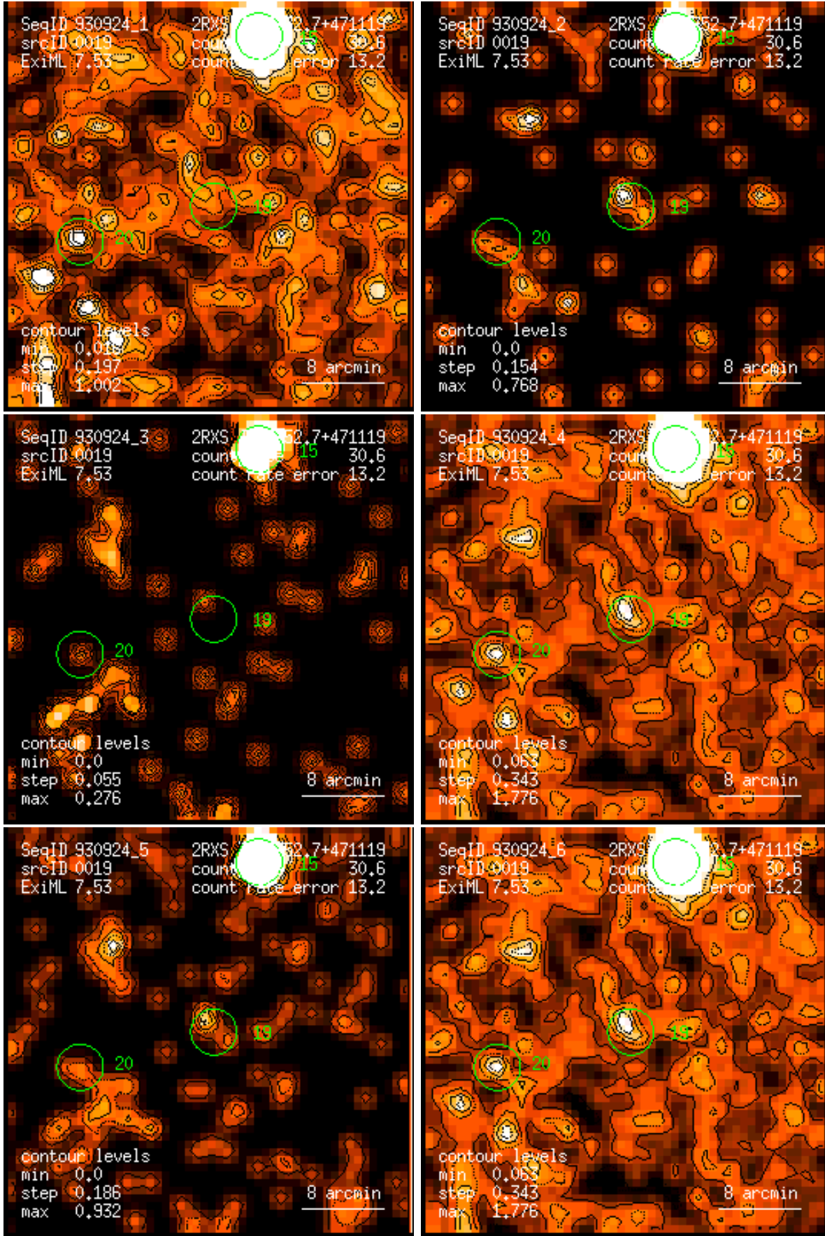
Figure 19: RASS 930924: detection 0019: band rate images, Gaussian filter: (1) PSPC channels 11 – 41, (2) 52 – 90, (3) 91 – 201, (4) 11 – 235, (5) 52 – 201, (6) 11 – 201. Broad band rates in counts/ks. Band rate contour levels in counts/ks/arcmin 2 .
