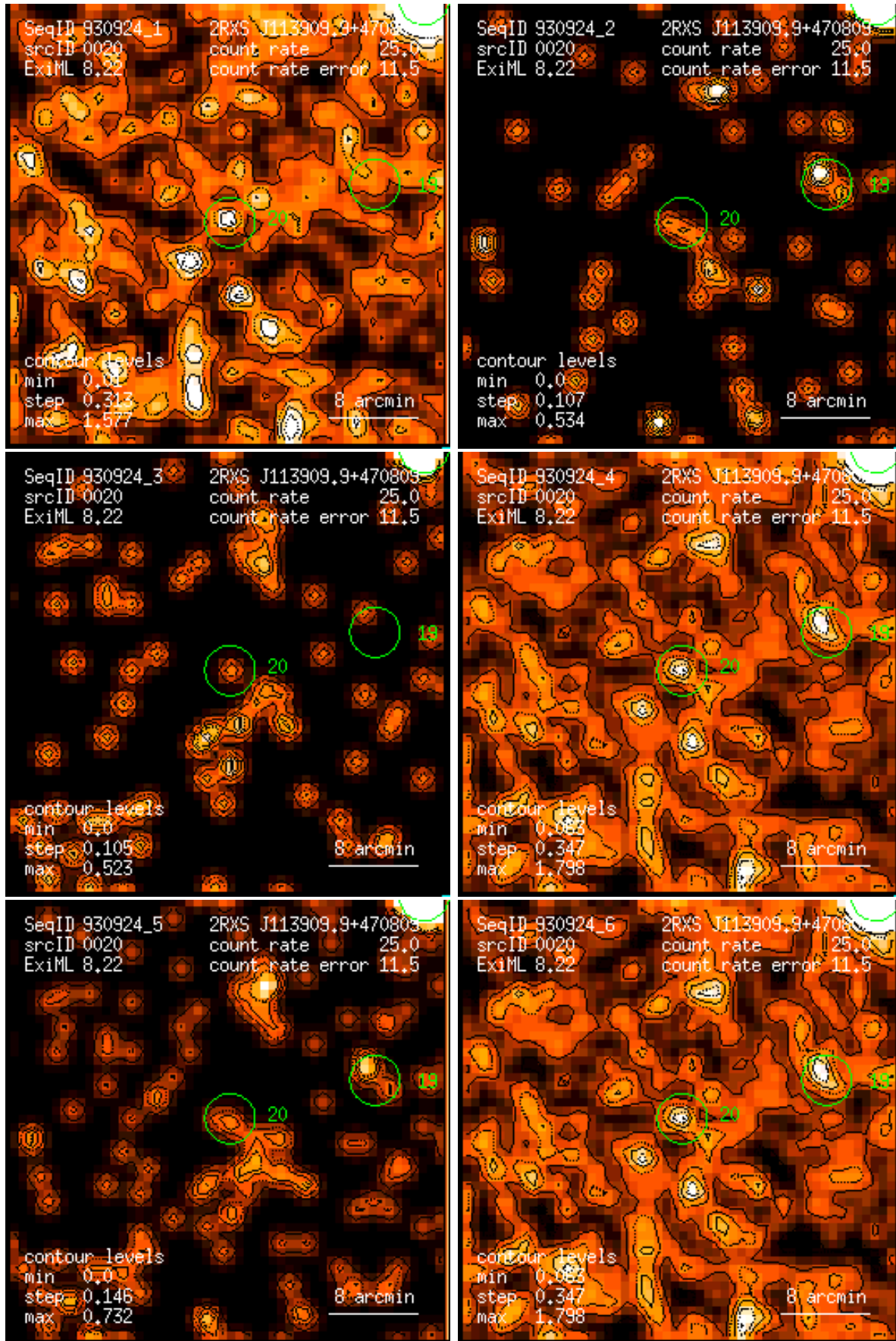
Figure 20: RASS 930924: detection 0020: band rate images, Gaussian filter: (1) PSPC channels 11 – 41, (2) 52 – 90, (3) 91 – 201, (4) 11 – 235, (5) 52 – 201, (6) 11 – 201. Broad band rates in counts/ks. Band rate contour levels in counts/ks/arcmin 2 .
