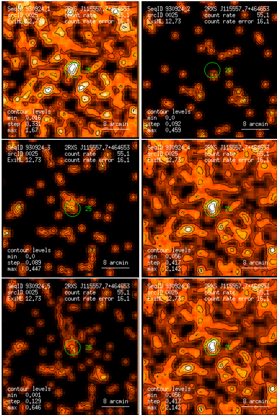
Figure 25: RASS 930924: detection 0025: band rate images, Gaussian filter: (1) PSPC channels 11 – 41, (2) 52 – 90, (3) 91 – 201, (4) 11 – 235, (5) 52 – 201, (6) 11 – 201. Broad band rates in counts/ks. Band rate contour levels in counts/ks/arcmin 2 .
