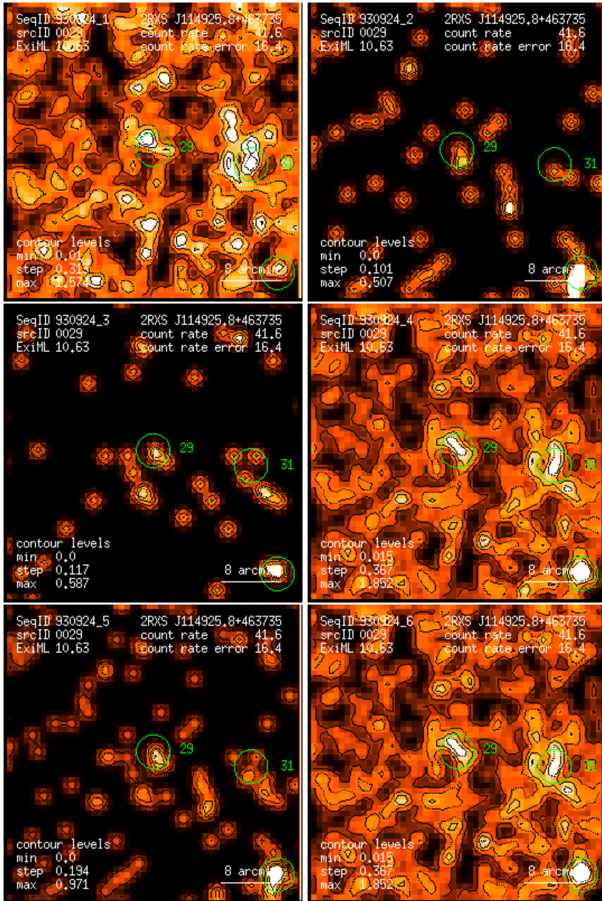
Figure 29: RASS 930924: detection 0029: band rate images, Gaussian filter: (1) PSPC channels 11 – 41, (2) 52 – 90, (3) 91 – 201, (4) 11 – 235, (5) 52 – 201, (6) 11 – 201. Broad band rates in counts/ks. Band rate contour levels in counts/ks/arcmin 2 .
