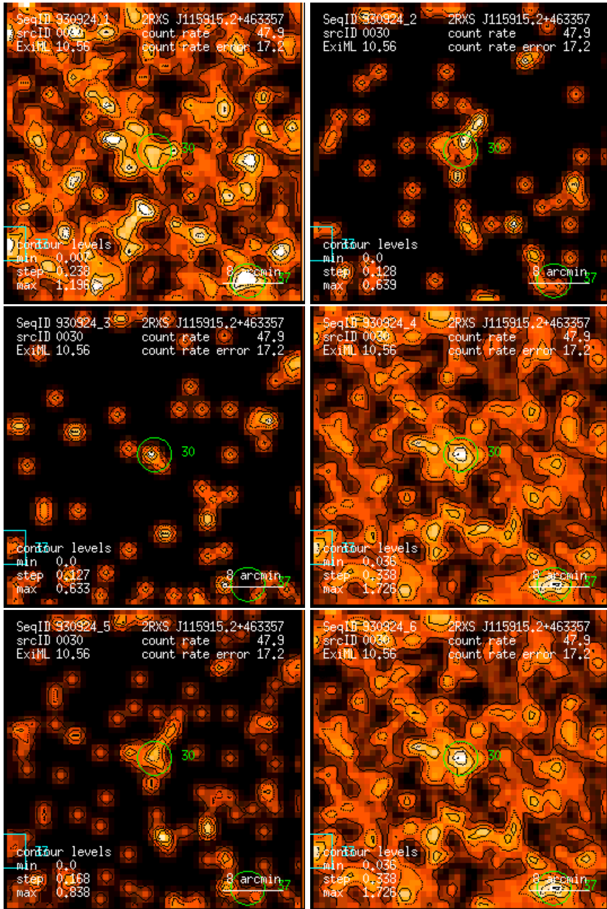
Figure 30: RASS 930924: detection 0030: band rate images, Gaussian filter: (1) PSPC channels 11 – 41, (2) 52 – 90, (3) 91 – 201, (4) 11 – 235, (5) 52 – 201, (6) 11 – 201. Broad band rates in counts/ks. Band rate contour levels in counts/ks/arcmin 2 .
