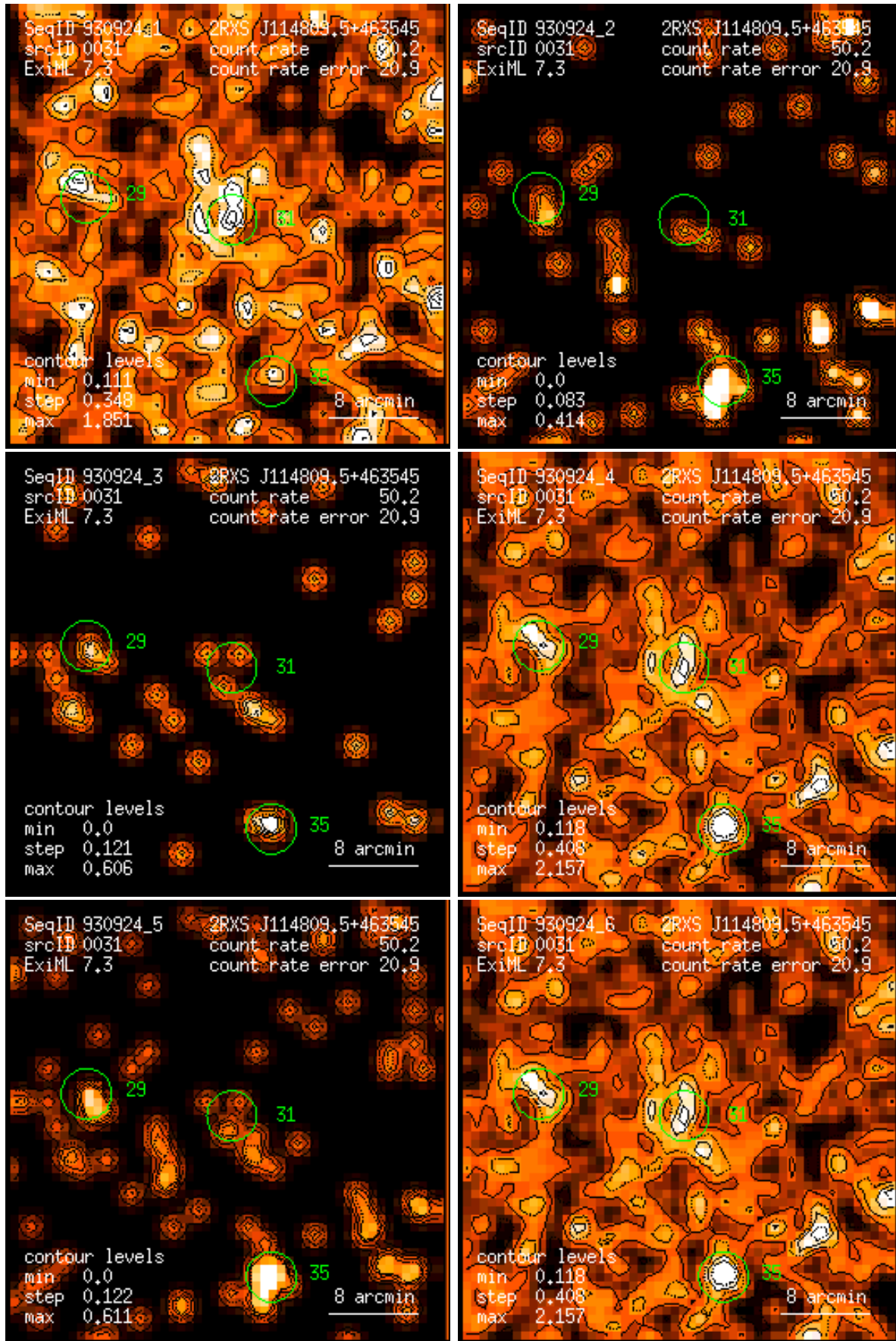
Figure 31: RASS 930924: detection 0031: band rate images, Gaussian filter: (1) PSPC channels 11 – 41, (2) 52 – 90, (3) 91 – 201, (4) 11 – 235, (5) 52 – 201, (6) 11 – 201. Broad band rates in counts/ks. Band rate contour levels in counts/ks/arcmin 2 .
