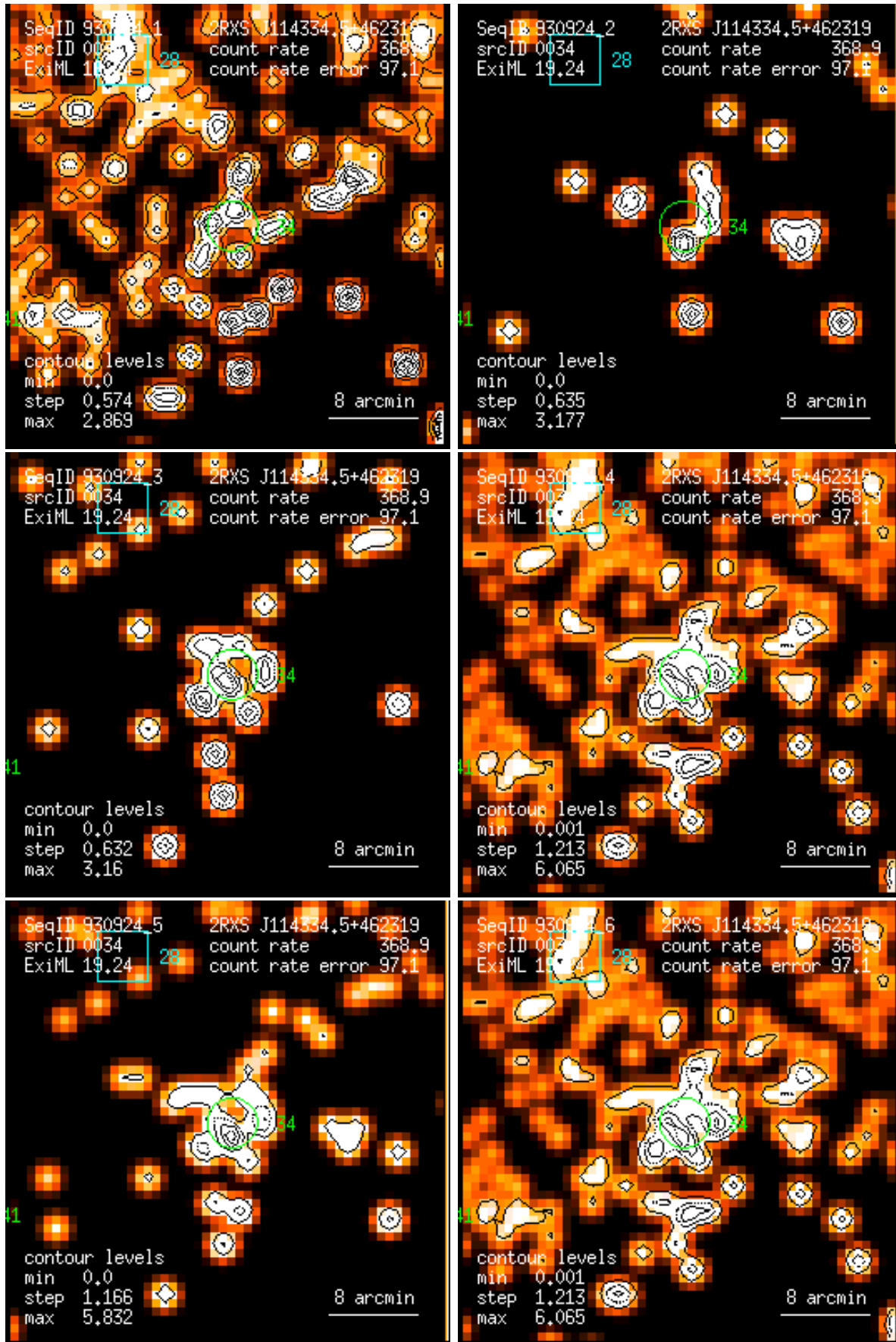
Figure 34: RASS 930924: detection 0034: band rate images, Gaussian filter: (1) PSPC channels 11 – 41, (2) 52 – 90, (3) 91 – 201, (4) 11 – 235, (5) 52 – 201, (6) 11 – 201. Broad band rates in counts/ks. Band rate contour levels in counts/ks/arcmin 2 .
