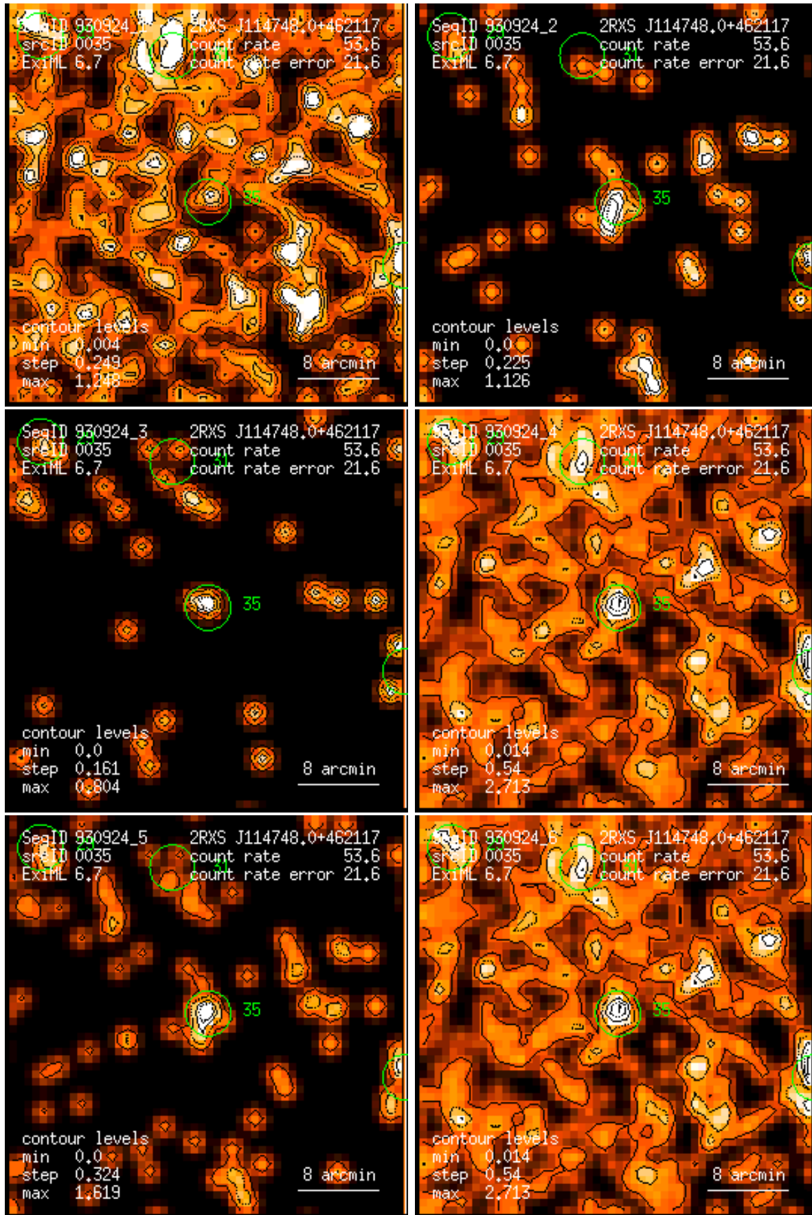
Figure 35: RASS 930924: detection 0035: band rate images, Gaussian filter: (1) PSPC channels 11 – 41, (2) 52 – 90, (3) 91 – 201, (4) 11 – 235, (5) 52 – 201, (6) 11 – 201. Broad band rates in counts/ks. Band rate contour levels in counts/ks/arcmin 2 .
