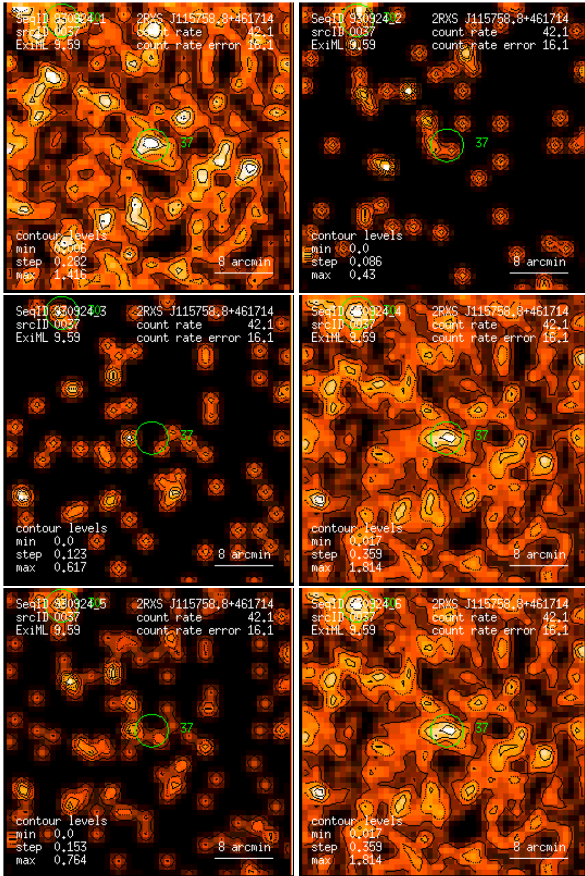
Figure 37: RASS 930924: detection 0037: band rate images, Gaussian filter: (1) PSPC channels 11 – 41, (2) 52 – 90, (3) 91 – 201, (4) 11 – 235, (5) 52 – 201, (6) 11 – 201. Broad band rates in counts/ks. Band rate contour levels in counts/ks/arcmin 2 .
