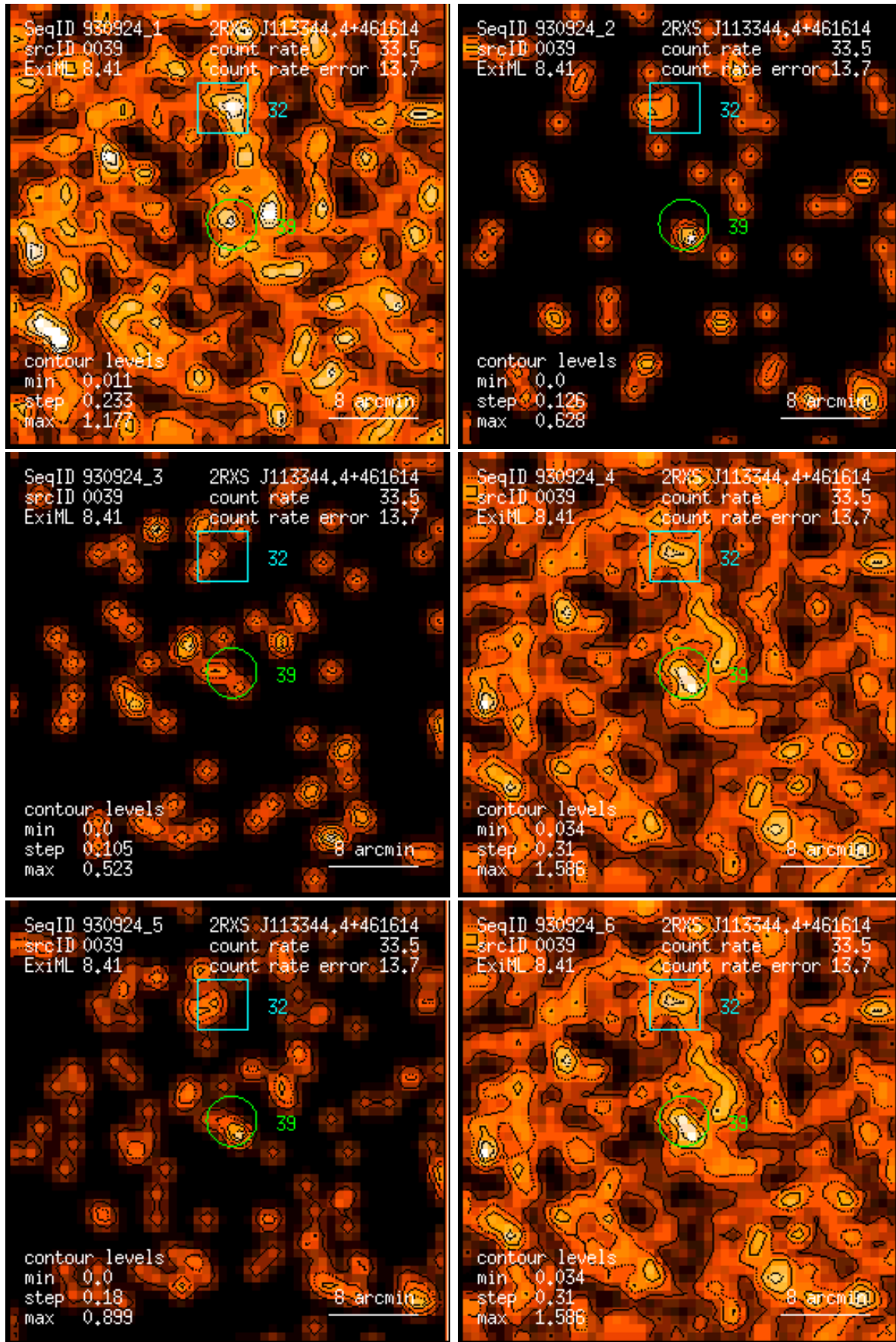
Figure 39: RASS 930924: detection 0039: band rate images, Gaussian filter: (1) PSPC channels 11 – 41, (2) 52 – 90, (3) 91 – 201, (4) 11 – 235, (5) 52 – 201, (6) 11 – 201. Broad band rates in counts/ks. Band rate contour levels in counts/ks/arcmin 2 .
