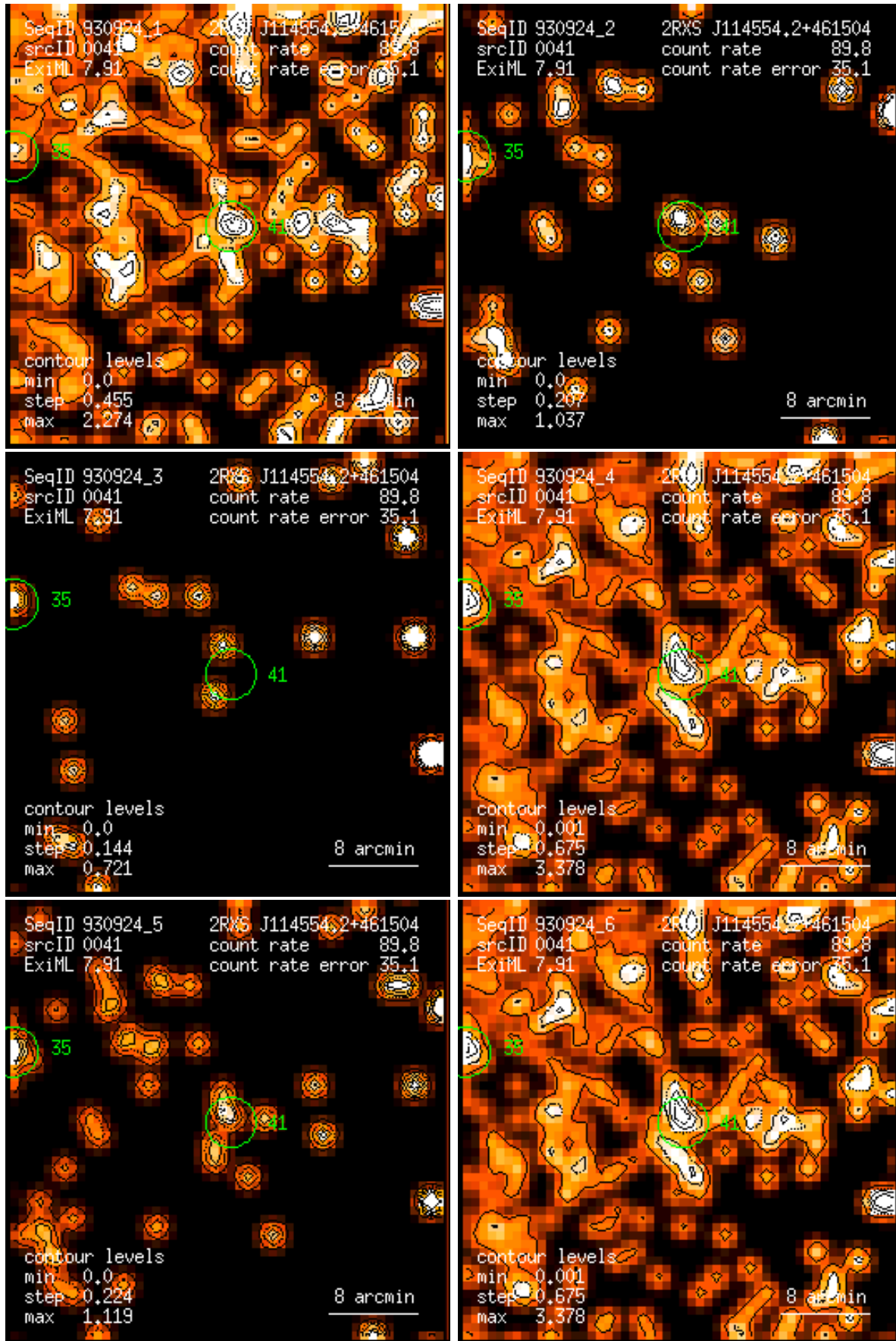
Figure 41: RASS 930924: detection 0041: band rate images, Gaussian filter: (1) PSPC channels 11 – 41, (2) 52 – 90, (3) 91 – 201, (4) 11 – 235, (5) 52 – 201, (6) 11 – 201. Broad band rates in counts/ks. Band rate contour levels in counts/ks/arcmin 2 .
