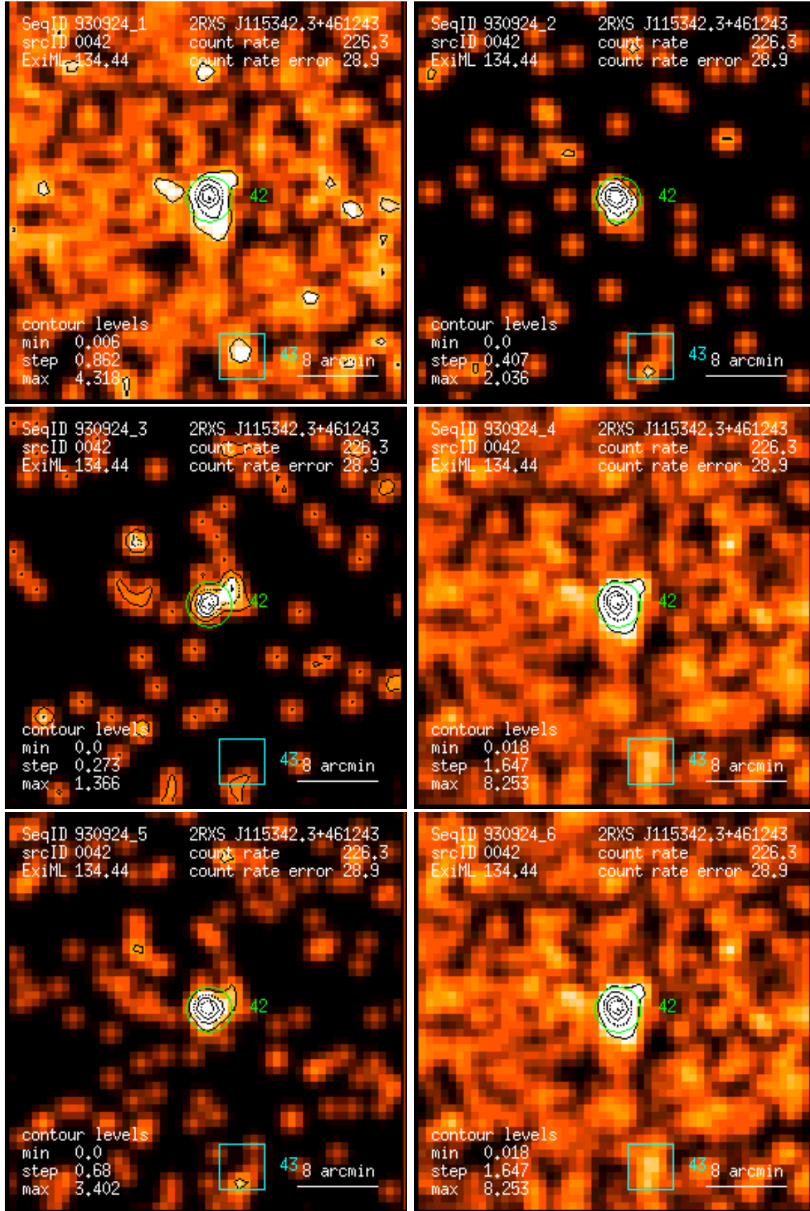
Figure 42: RASS 930924: detection 0042: band rate images, Gaussian filter: (1) PSPC channels 11 – 41, (2) 52 – 90, (3) 91 – 201, (4) 11 – 235, (5) 52 – 201, (6) 11 – 201. Broad band rates in counts/ks. Band rate contour levels in counts/ks/arcmin 2 .
