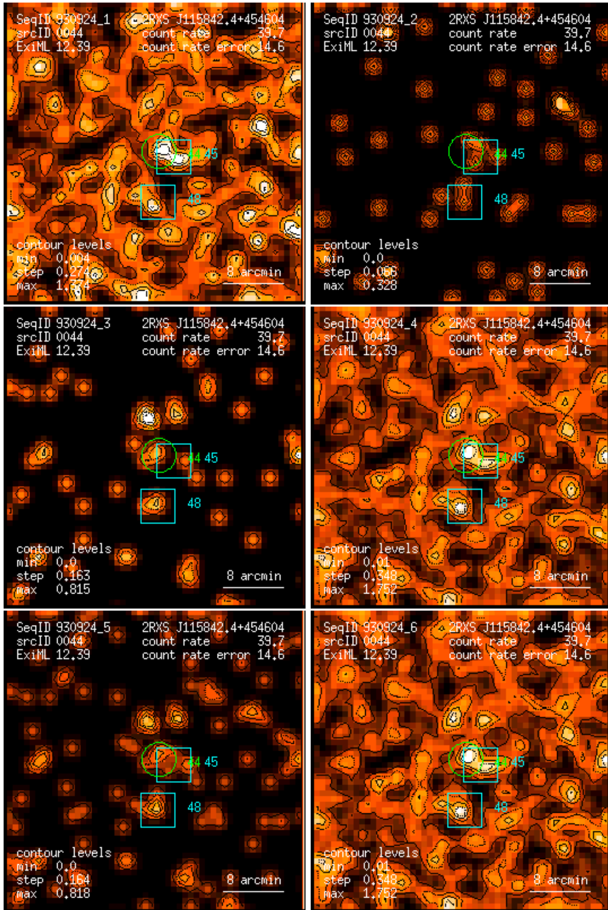
Figure 44: RASS 930924: detection 0044: band rate images, Gaussian filter: (1) PSPC channels 11 – 41, (2) 52 – 90, (3) 91 – 201, (4) 11 – 235, (5) 52 – 201, (6) 11 – 201. Broad band rates in counts/ks. Band rate contour levels in counts/ks/arcmin 2 .
