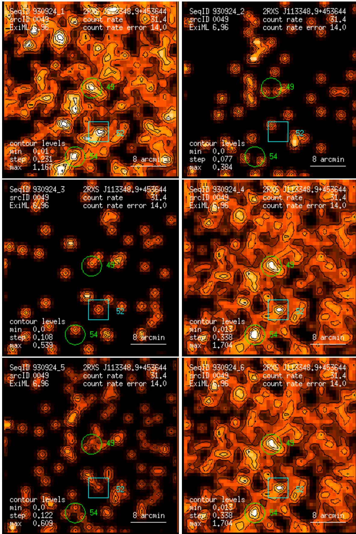
Figure 49: RASS 930924: detection 0049: band rate images, Gaussian filter: (1) PSPC channels 11 – 41, (2) 52 – 90, (3) 91 – 201, (4) 11 – 235, (5) 52 – 201, (6) 11 – 201. Broad band rates in counts/ks. Band rate contour levels in counts/ks/arcmin 2 .
