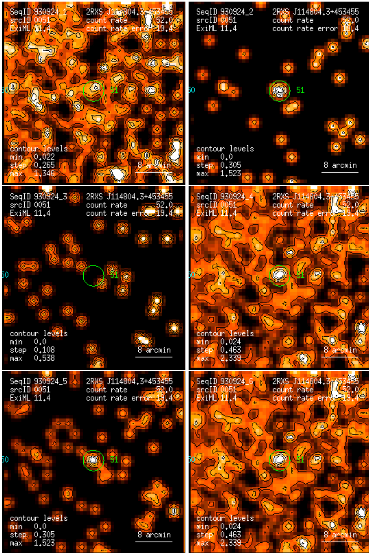
Figure 51: RASS 930924: detection 0051: band rate images, Gaussian filter: (1) PSPC channels 11 – 41, (2) 52 – 90, (3) 91 – 201, (4) 11 – 235, (5) 52 – 201, (6) 11 – 201. Broad band rates in counts/ks. Band rate contour levels in counts/ks/arcmin 2 .
