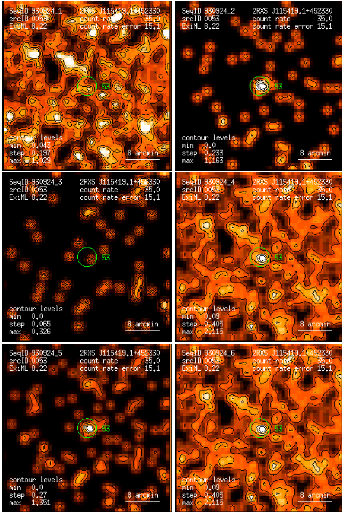
Figure 53: RASS 930924: detection 0053: band rate images, Gaussian filter: (1) PSPC channels 11 – 41, (2) 52 – 90, (3) 91 – 201, (4) 11 – 235, (5) 52 – 201, (6) 11 – 201. Broad band rates in counts/ks. Band rate contour levels in counts/ks/arcmin 2 .
