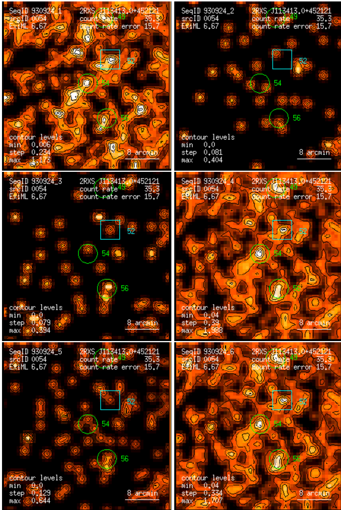
Figure 54: RASS 930924: detection 0054: band rate images, Gaussian filter: (1) PSPC channels 11 – 41, (2) 52 – 90, (3) 91 – 201, (4) 11 – 235, (5) 52 – 201, (6) 11 – 201. Broad band rates in counts/ks. Band rate contour levels in counts/ks/arcmin 2 .
