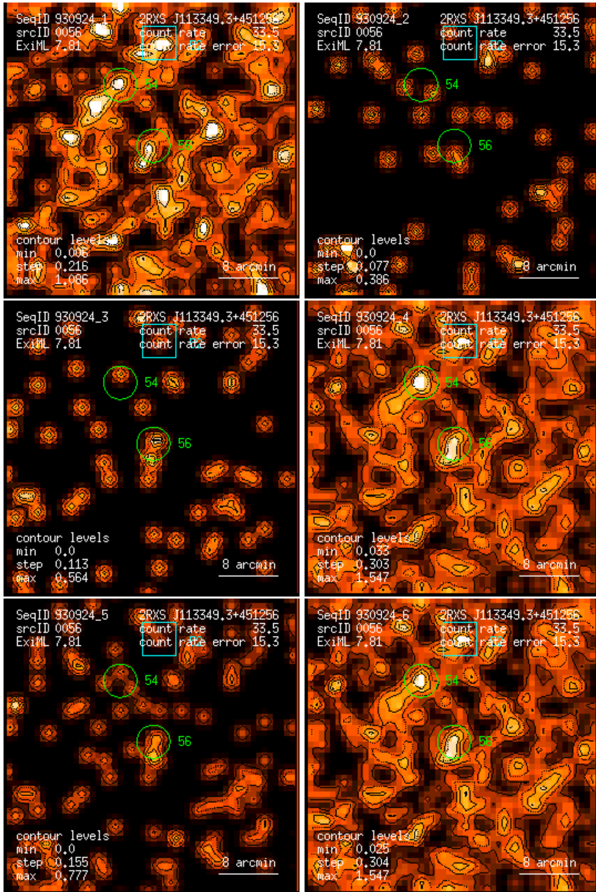
Figure 56: RASS 930924: detection 0056: band rate images, Gaussian filter: (1) PSPC channels 11 – 41, (2) 52 – 90, (3) 91 – 201, (4) 11 – 235, (5) 52 – 201, (6) 11 – 201. Broad band rates in counts/ks. Band rate contour levels in counts/ks/arcmin 2 .
