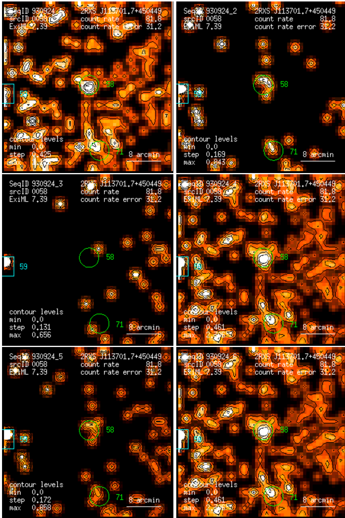
Figure 58: RASS 930924: detection 0058: band rate images, Gaussian filter: (1) PSPC channels 11 – 41, (2) 52 – 90, (3) 91 – 201, (4) 11 – 235, (5) 52 – 201, (6) 11 – 201. Broad band rates in counts/ks. Band rate contour levels in counts/ks/arcmin 2 .
