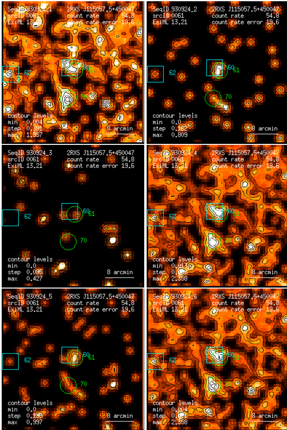
Figure 61: RASS 930924: detection 0061: band rate images, Gaussian filter: (1) PSPC channels 11 – 41, (2) 52 – 90, (3) 91 – 201, (4) 11 – 235, (5) 52 – 201, (6) 11 – 201. Broad band rates in counts/ks. Band rate contour levels in counts/ks/arcmin 2 .
