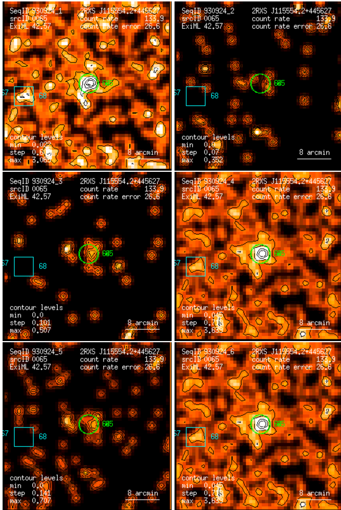
Figure 65: RASS 930924: detection 0065: band rate images, Gaussian filter: (1) PSPC channels 11 – 41, (2) 52 – 90, (3) 91 – 201, (4) 11 – 235, (5) 52 – 201, (6) 11 – 201. Broad band rates in counts/ks. Band rate contour levels in counts/ks/arcmin 2 .
