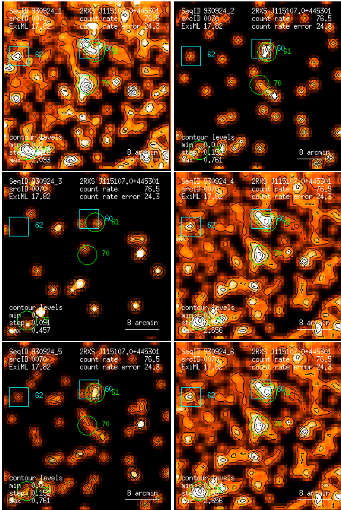
Figure 70: RASS 930924: detection 0070: band rate images, Gaussian filter: (1) PSPC channels 11 – 41, (2) 52 – 90, (3) 91 – 201, (4) 11 – 235, (5) 52 – 201, (6) 11 – 201. Broad band rates in counts/ks. Band rate contour levels in counts/ks/arcmin 2 .
